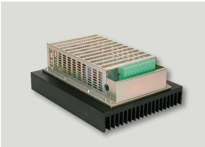
500W ruggedized AC/DC power supply for ship crane application. Single output 25.5V, input voltage range 115-230VAC.
