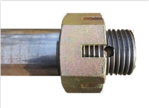
Press Axle - 50mm to 60mm Press Axles to suit Simba, Gallucho and others
