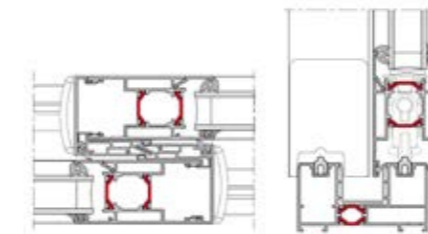
Dual Rail – Standard Interlock
