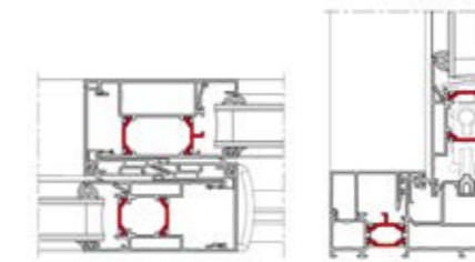
Mono Rail – Standard Interlock
