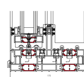
Sill Detail
