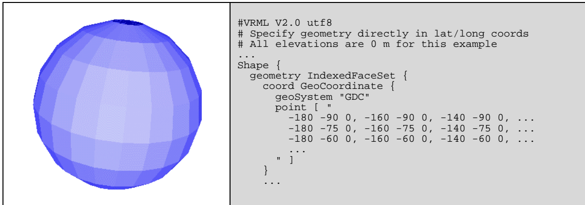
Figure 4: Illustrating the use of the GeoCoordinate node to insert latitude/longitude coordinates directly in a VRML file. These coordinates are transparently transformed to geocentric coordinates to produce an ellipsoidal model of the earth, as seen on the left.
