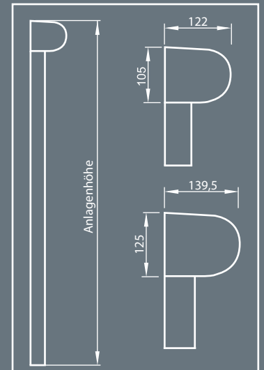
The round system SolidScreen® SGF
