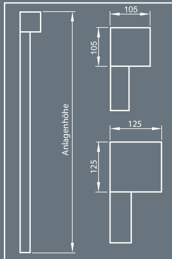
The square system SolidScreen® SG 90
