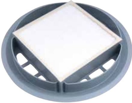
HEPA H13 filter capable of capturing 99.997% of particles down to 0.3 microns
