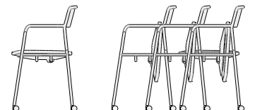
Horizontal stack By raising the seating surface, horizontally, You can stack it. (Stack pitch: 250 mm)
