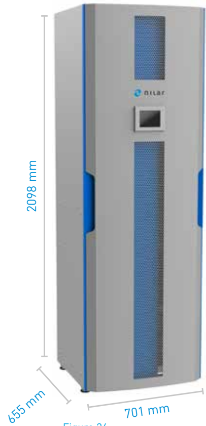
Figure 24. Cabinet 28,8 kWh
