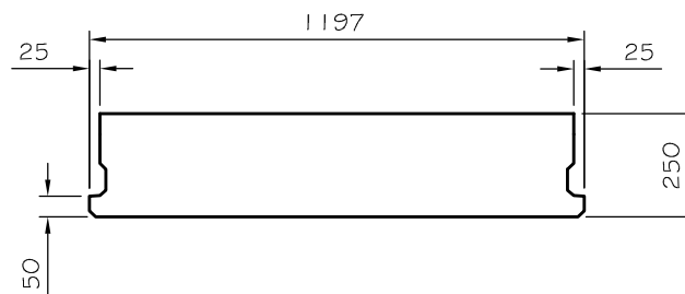
250mm DEEP WIDESLAB DIMENSIONS
