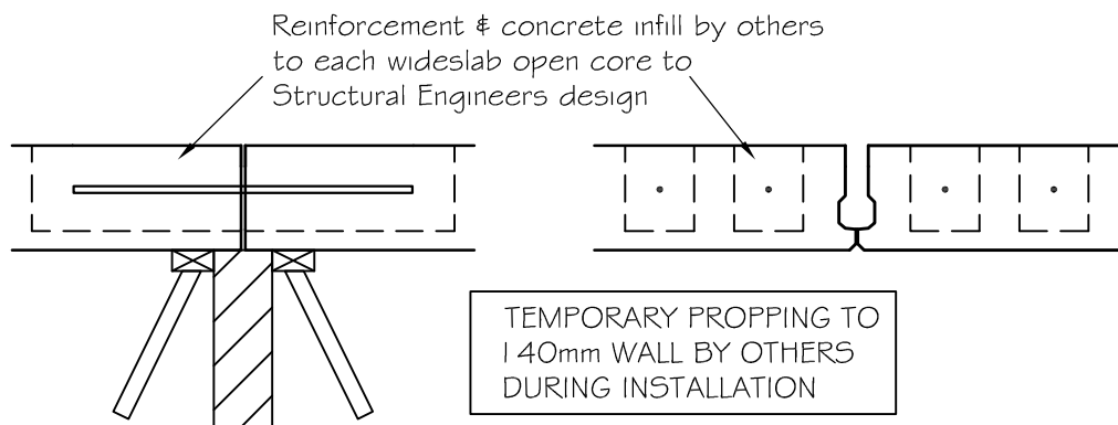
140mm SHARED BEARING WALL DETAIL
