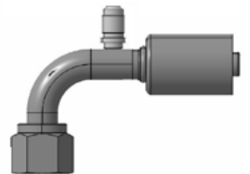
O-ring female swivel - pressure sensor 7/16-20 90° elbow
