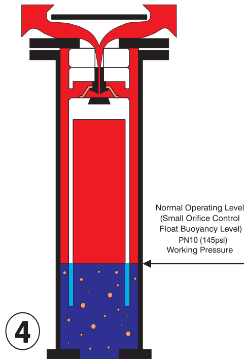
PRESSURIZED AIR / GAS RELEASE PIPELINE OPERATING
