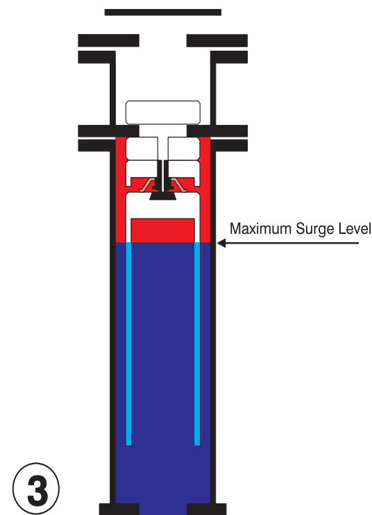
PIPELINE FULLY CHARGED
