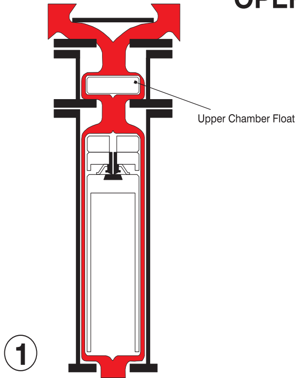
PIPELINE FILLING (SUB CRITICAL SEWAGE / EFFLUENT APPROACH VELOCITY)
