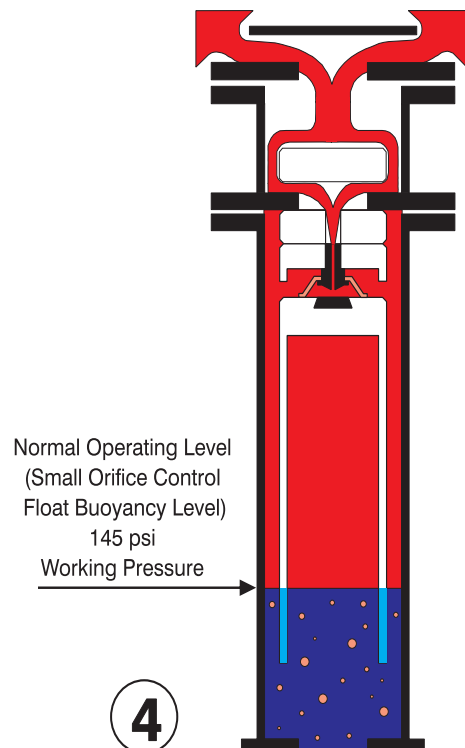
PRESSURIZED AIR/GAS RELEASE FROM A FULL PIPELINE
