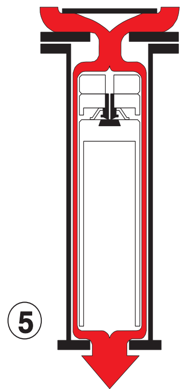
VACUUM RELIEF (AIR INTAKE) PIPELINE DRAINING
