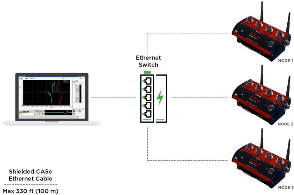
Figure 21: Wired Ethernet System Configuration using LAN Switch
