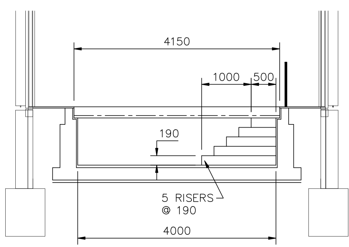
SECTION B-B
