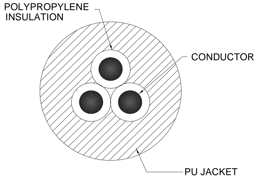
GEOPHONE LEADER CABLE (3 CORE)
