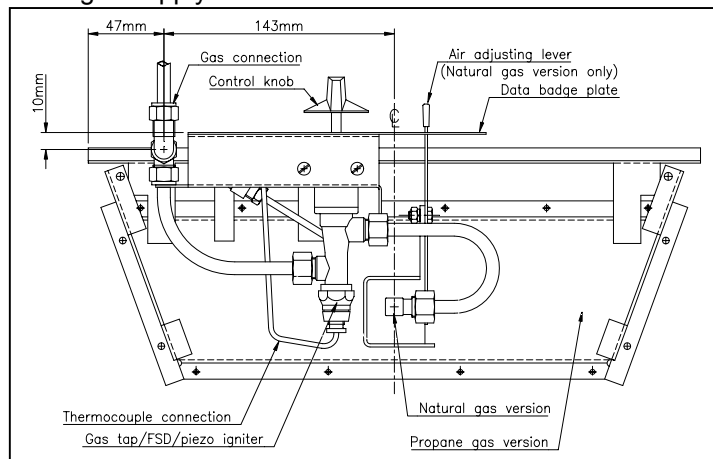
Fig. 11 Underside of burner
