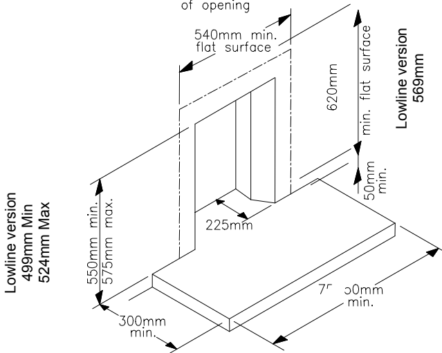
Fig.2c Pre-cast block flue
