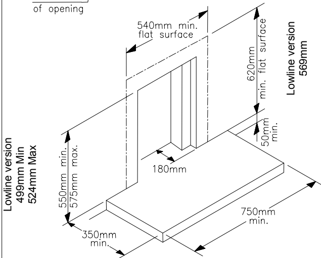
Fig.2d Pre-cast block flue used with spacing frame
