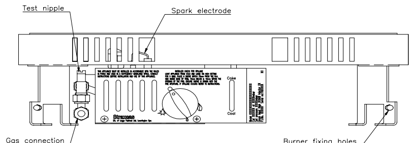
Fig. 8 The data badge plate & test
