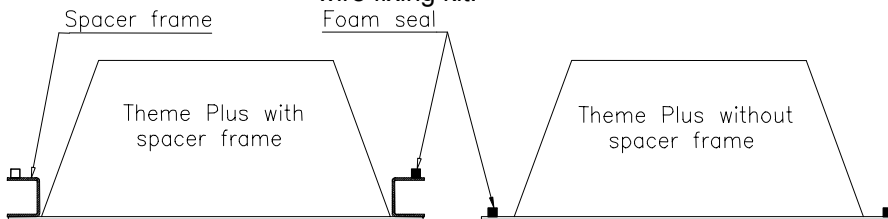
Fig.3a Attaching foam seal
