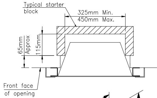
Fig.2b Masonry chimney without chairbrick
