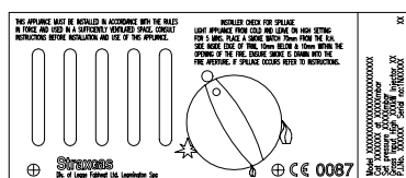
Fig.9 Data badge plate - propane version
