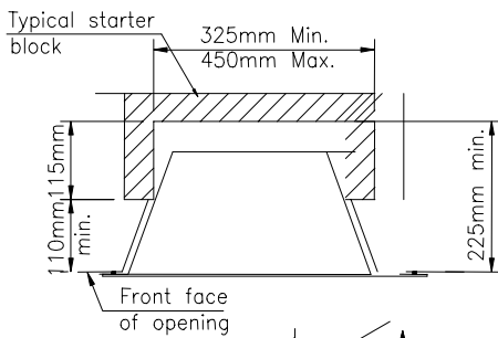
Fig.2a Masonry chimney with chairbrick
