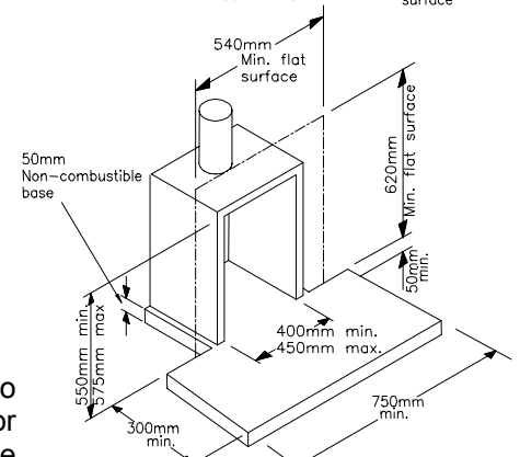
Fig.4 Metal fluebox and flue system
