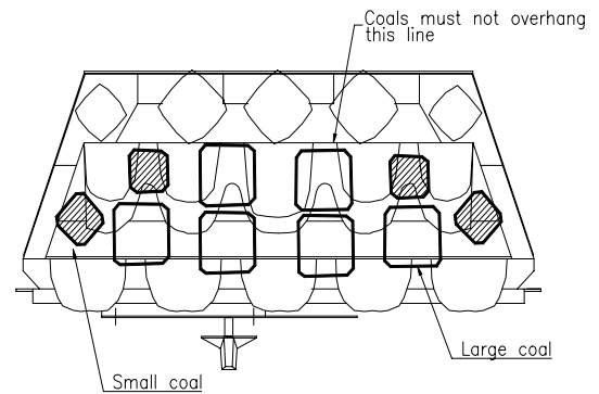
Fig.6 Placing the loose coals
