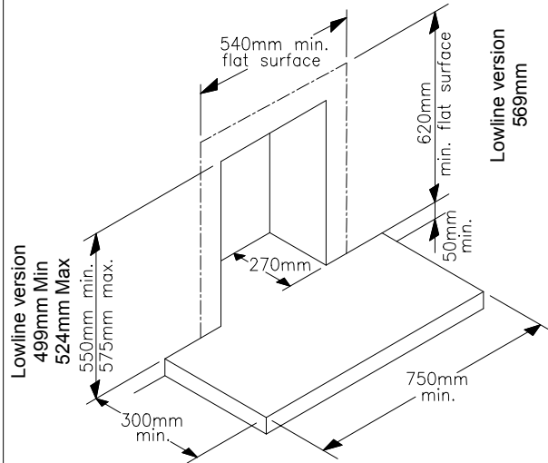
Fig.2b Masonry chimney without chairbrick
