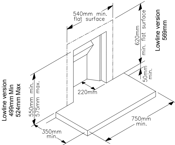
Fig.2a Masonry chimney with chairbrick
