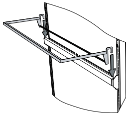
Attach Kwickload™ Cooler Baffle Frame to Adjustable Crossbar
