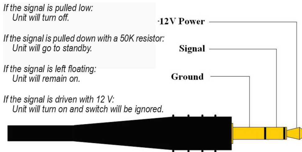
12 Volt Remote Trigger wiring.
