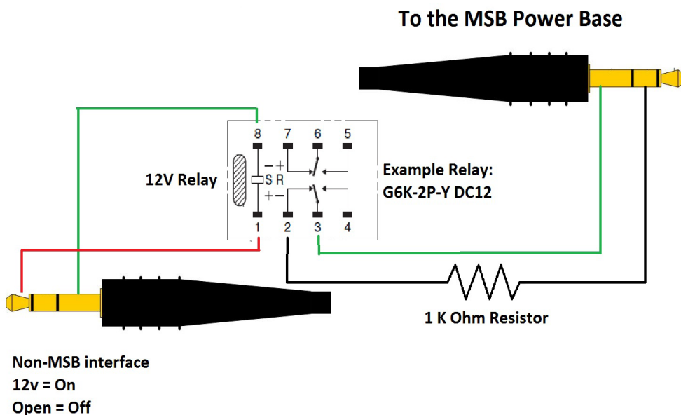
12 Volt Remote Trigger wiring.
