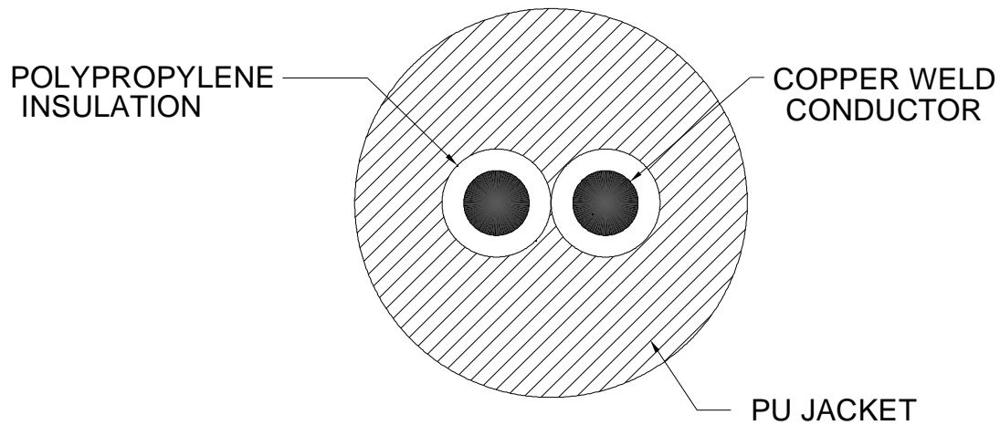
GEOPHONE LEADER CABLE(2 CORE)
