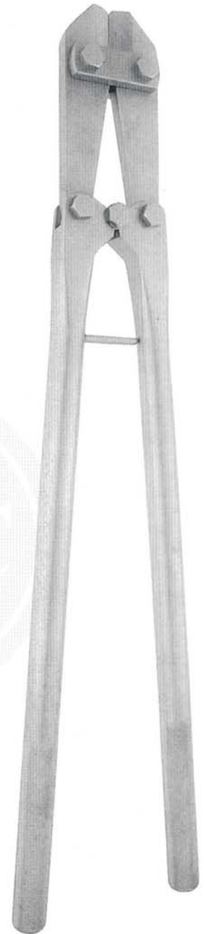
130-246-60 Cutter for cutting of Kirschner wire Sreimann Pins up to 6 mm Ø har 460 mm TC
