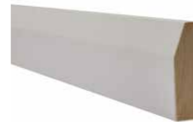
WHITE CHAMFERED ARCHITRAVE Material White Primed Size 18 x 70mm Code WFCHARC1870
