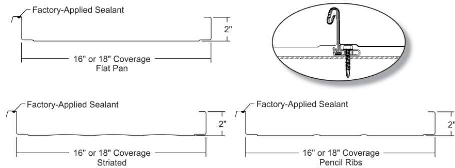
FIGURE 2A—MAGNA-LOC 180
