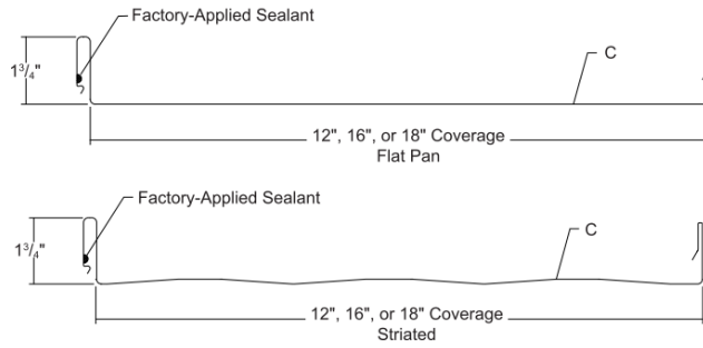
FIGURE 3A—VERTICAL SEAM
