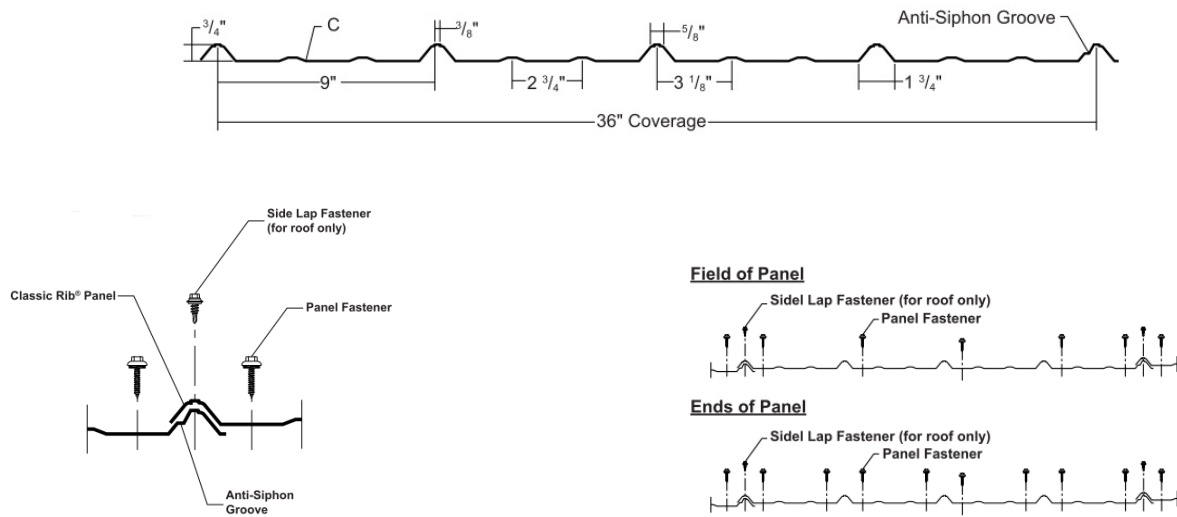
FIGURE 8—CLASSIC RIB
