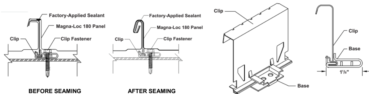
FIGURE 2B—MAGNA-LOC CLIP
