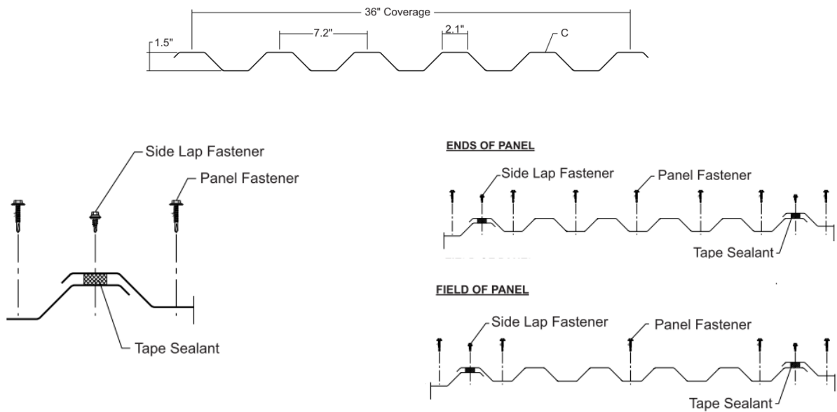
FIGURE 6—IC72 PANEL
