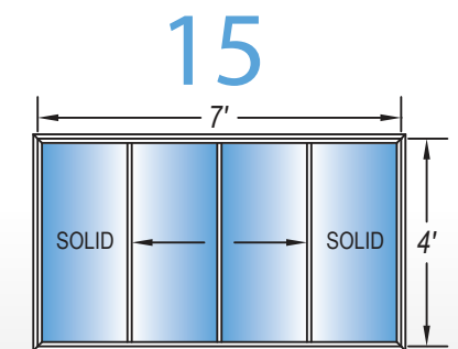
2 Stationary Windows 2 Horizontal Sliders
