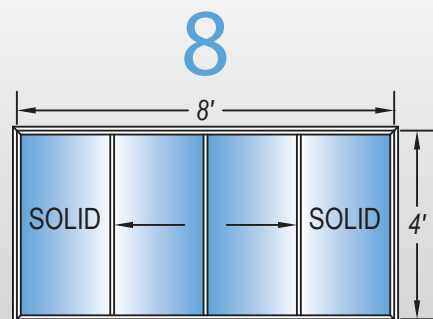
2 Stationary Windows 2 Horizontal Sliders
