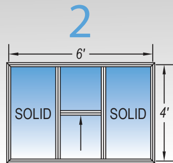
2 Stationary Windows 1 Vertical Slider
