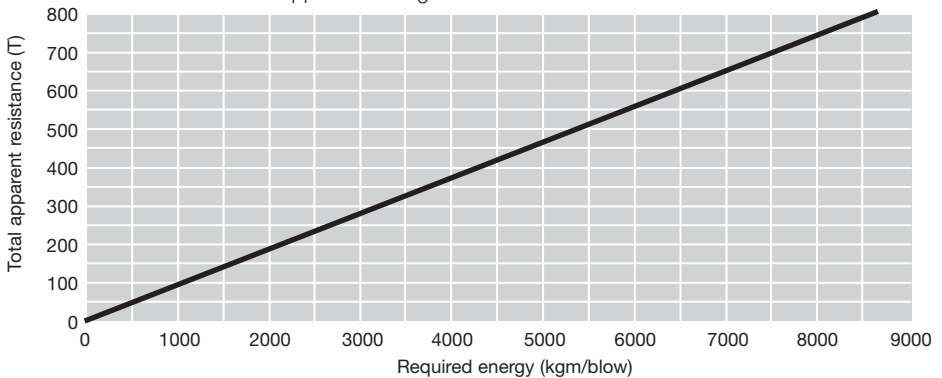
Fig 11.6.4 Relationship between required delivered energy and apparent driving resistance near refusal
