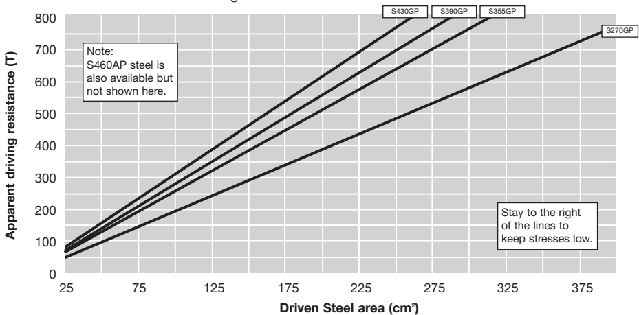
Fig 11.6.5 Minimum steel area to be driven for a given apparent driving resistance
