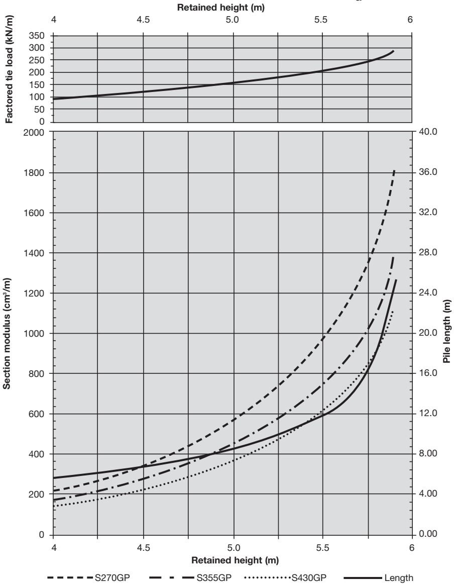
Fig. 8.33 Tied - Water condition C (d = 1.2m) S_u = 40\text{kN/m}^2
