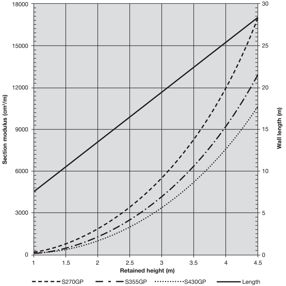
Fig. 8.12 Cantilever - Water condition A
