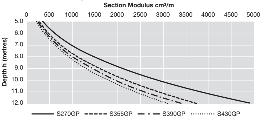
Fig 7.7.2 Depth v Section Modulus
