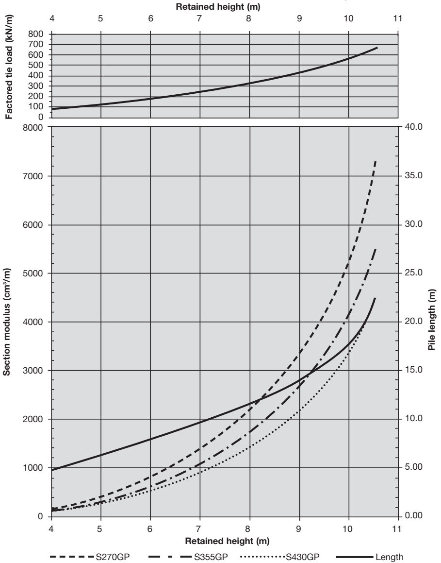
Fig. 8.32 Tied - Water condition C (d=1.2m) S_u = 75\text{kN/m}^2
