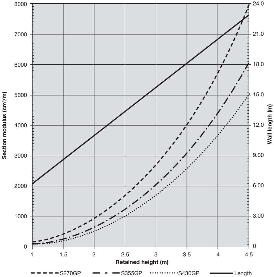
Fig. 8.15 Cantilever - Water condition B
