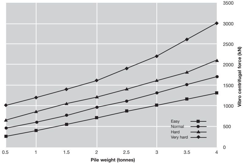
Fig 11.6.9 Guidance for size of vibrohammer (rated by centrifugal force) in terms of pile weight and driving conditions
