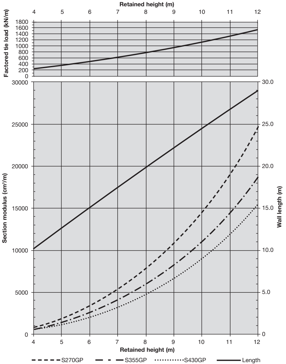
Fig. 8.24 Tied - Water condition B (d=1.5m)
