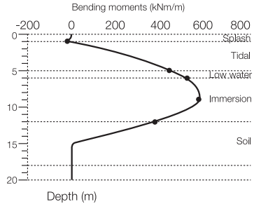
Fig 3.4b Typical marine wall bending moments
