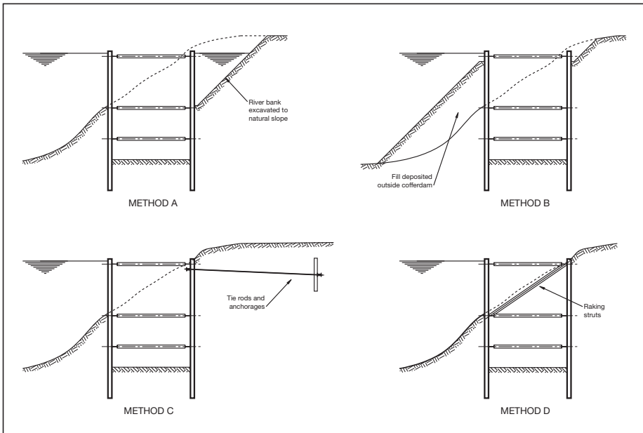
Fig 7.8.2 Construction of cofferdams in river banks
