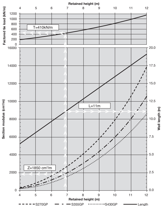
Fig. 8.9 Example plot
