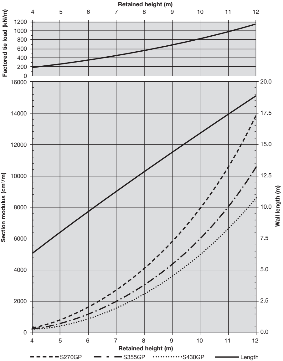
Fig. 8.19 Tied - Water condition A (d=1.5m)
