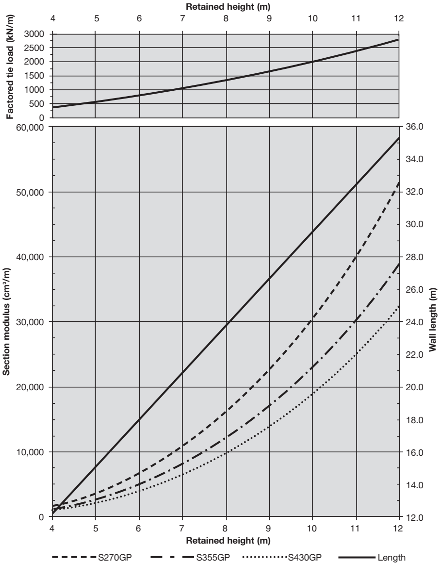
Fig. 8.21 Tied - Water condition A (d=1.5m)
