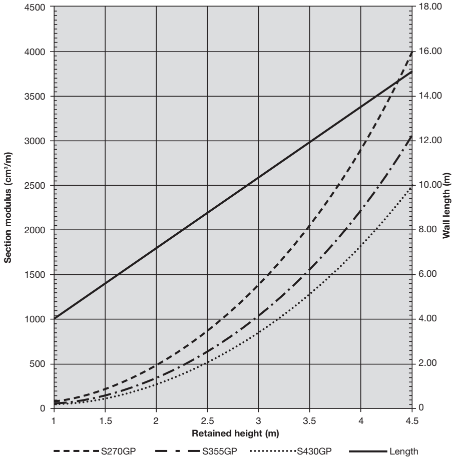
Fig. 8.18 Cantilever - Water condition C
