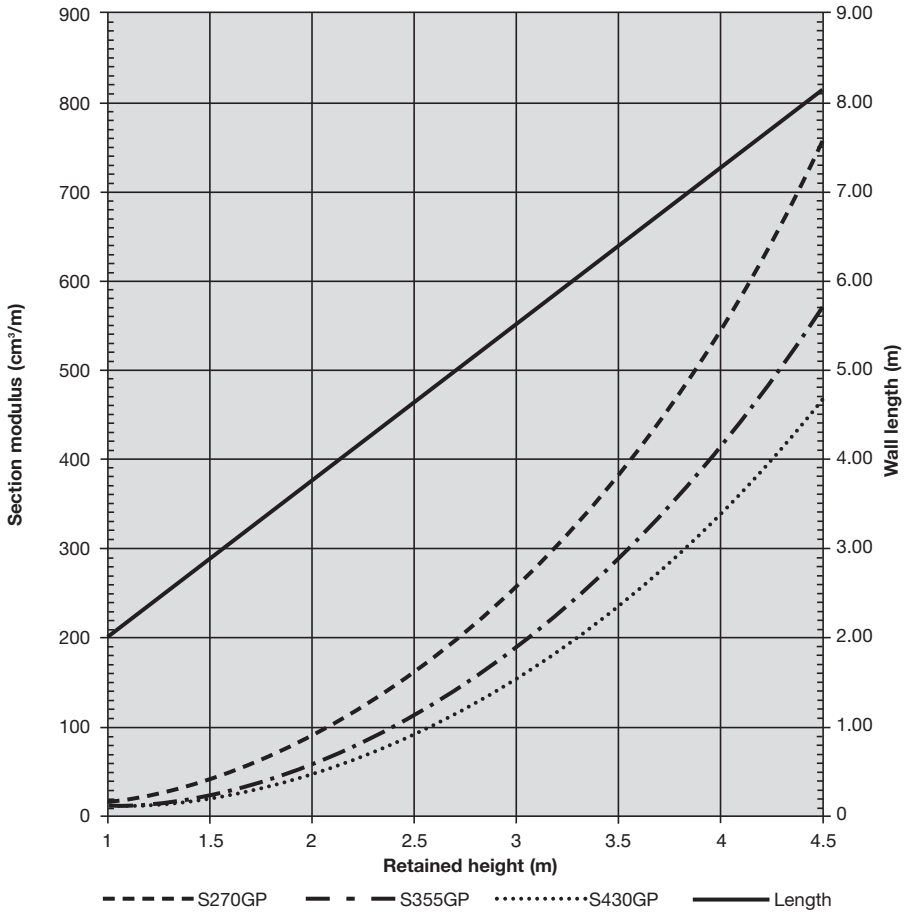
Fig. 8.16 Cantilever - Water condition C
