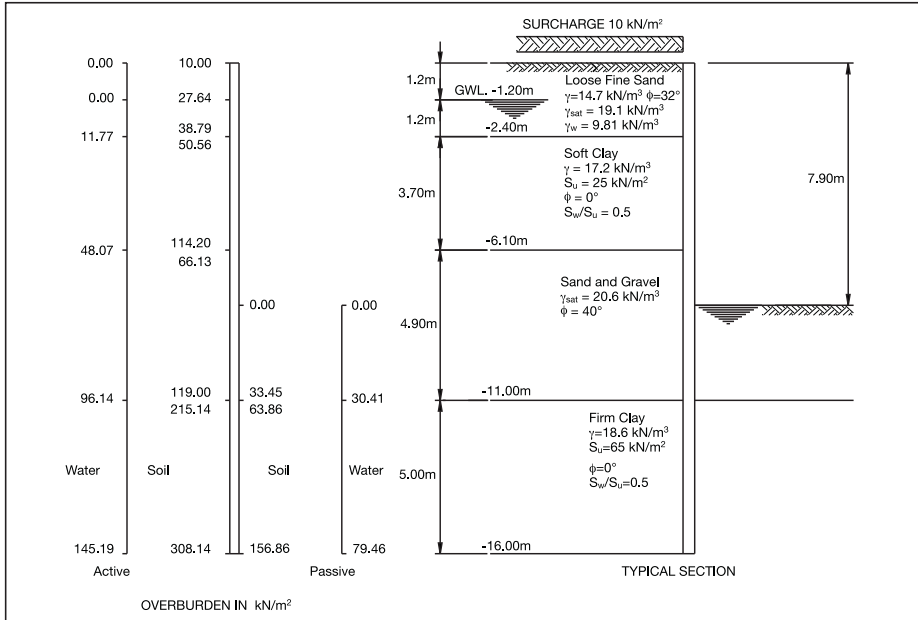
Fig 4.16.1 Total Stress Analysis Example
