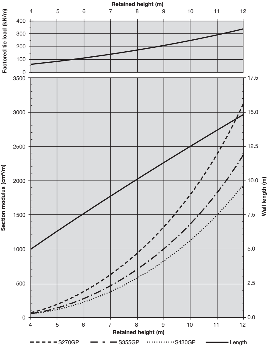
Fig. 8.25 Tied - Water condition C (d=1.5m)
