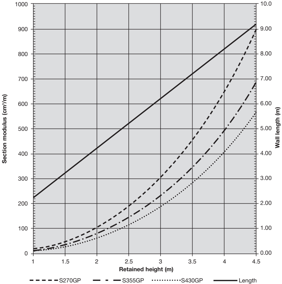
Fig. 8.13 Cantilever - Water condition B
