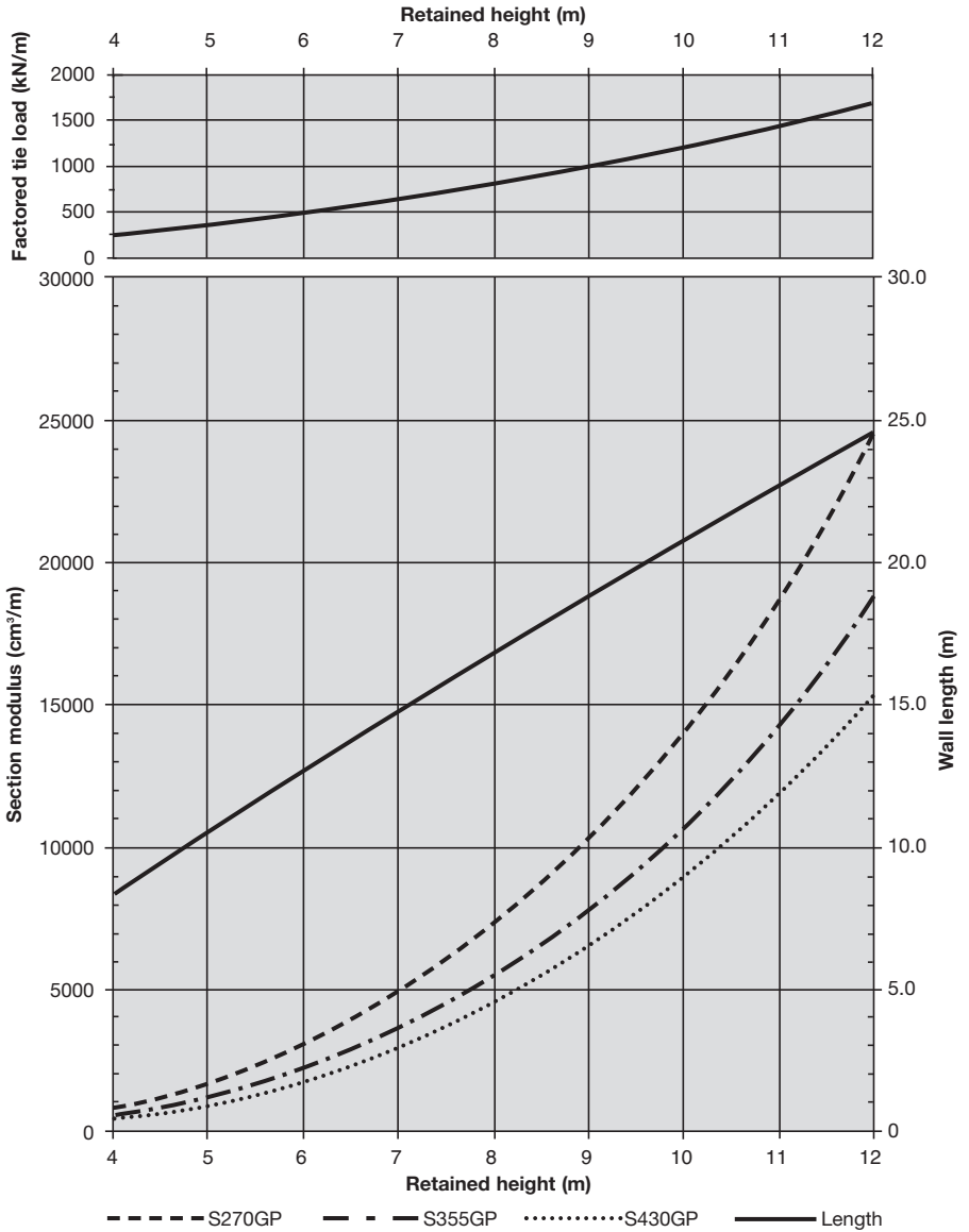
Fig. 8.20 Tied - Water condition A (d=1.5m)
