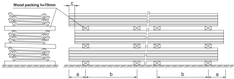
Fig 9.9a Storage of straight-web sheet piles
