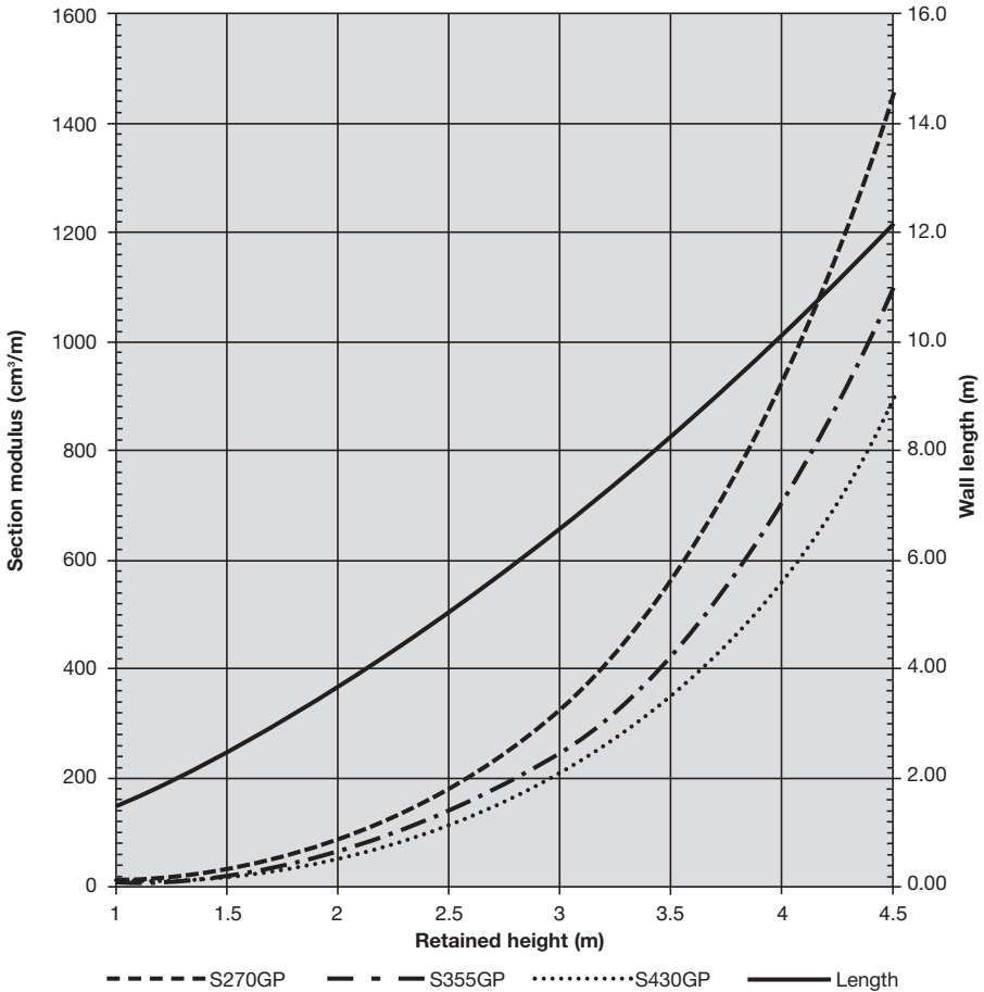
Fig. 8.31 Cantilever - Water condition D S_u = 40\text{kN/m}^2
