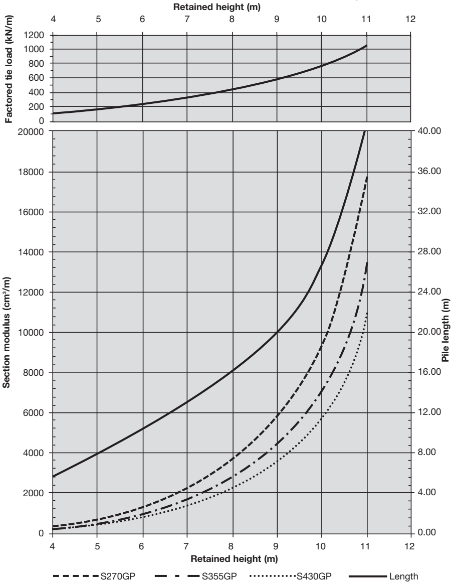
Fig. 8.35 Tied - Water condition D (d=1.2m) S_u = 40\text{kN/m}^2
