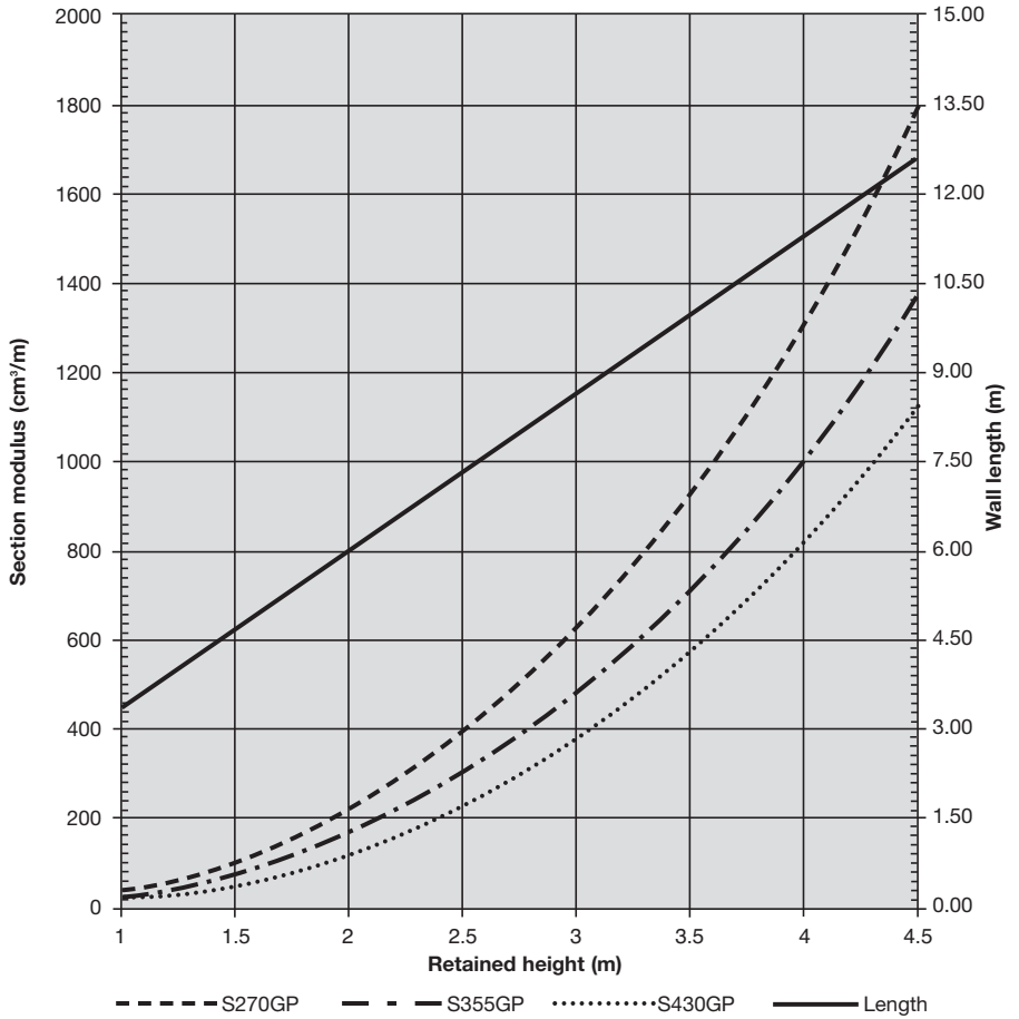
Fig. 8.14 Cantilever - Water condition B
