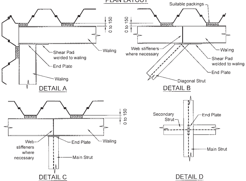
PLAN LAYOUT
