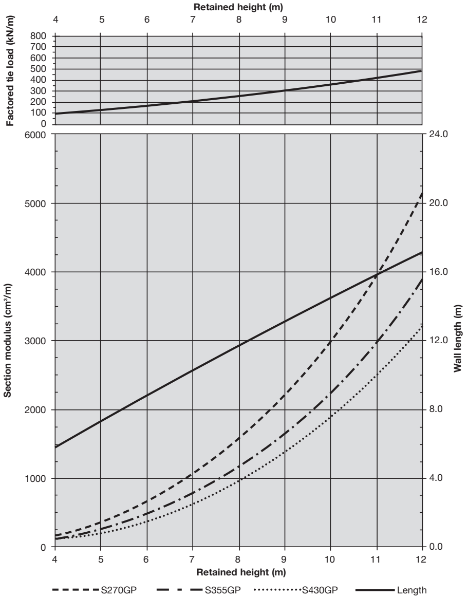
Fig. 8.26 Tied - Water condition C (d=1.5m)
