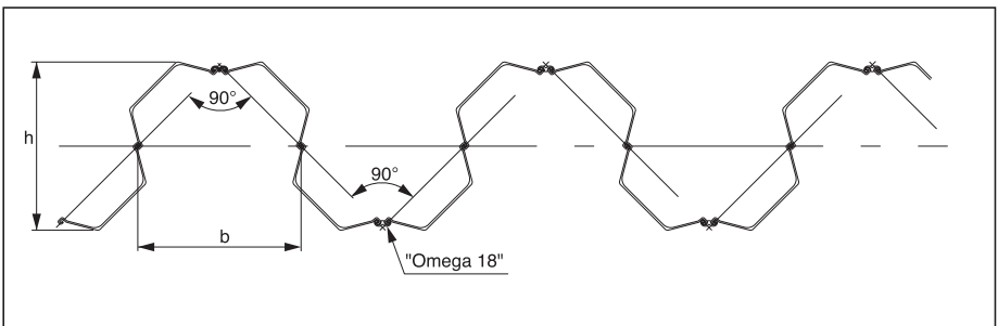
Fig 1.16.6b U Jagged wall
