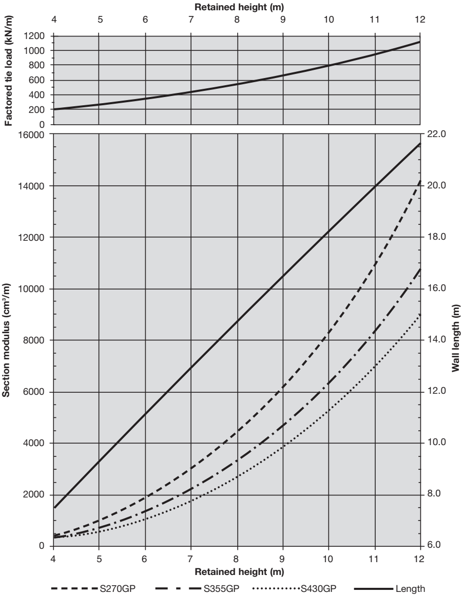
Fig. 8.27 Tied - Water condition C (d=1.5m)
