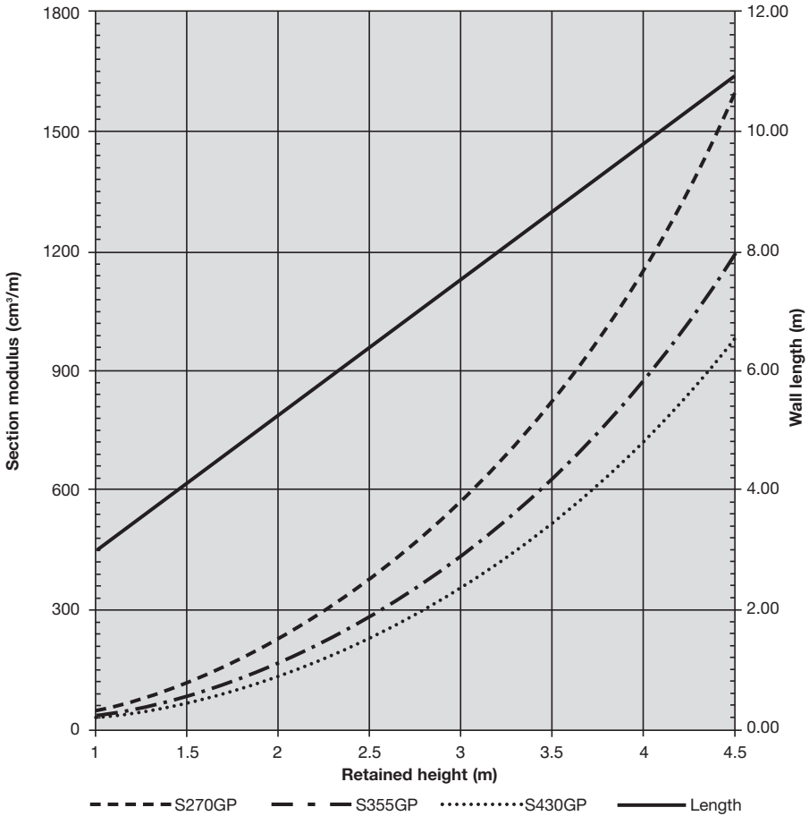
Fig. 8.17 Cantilever - Water condition C
