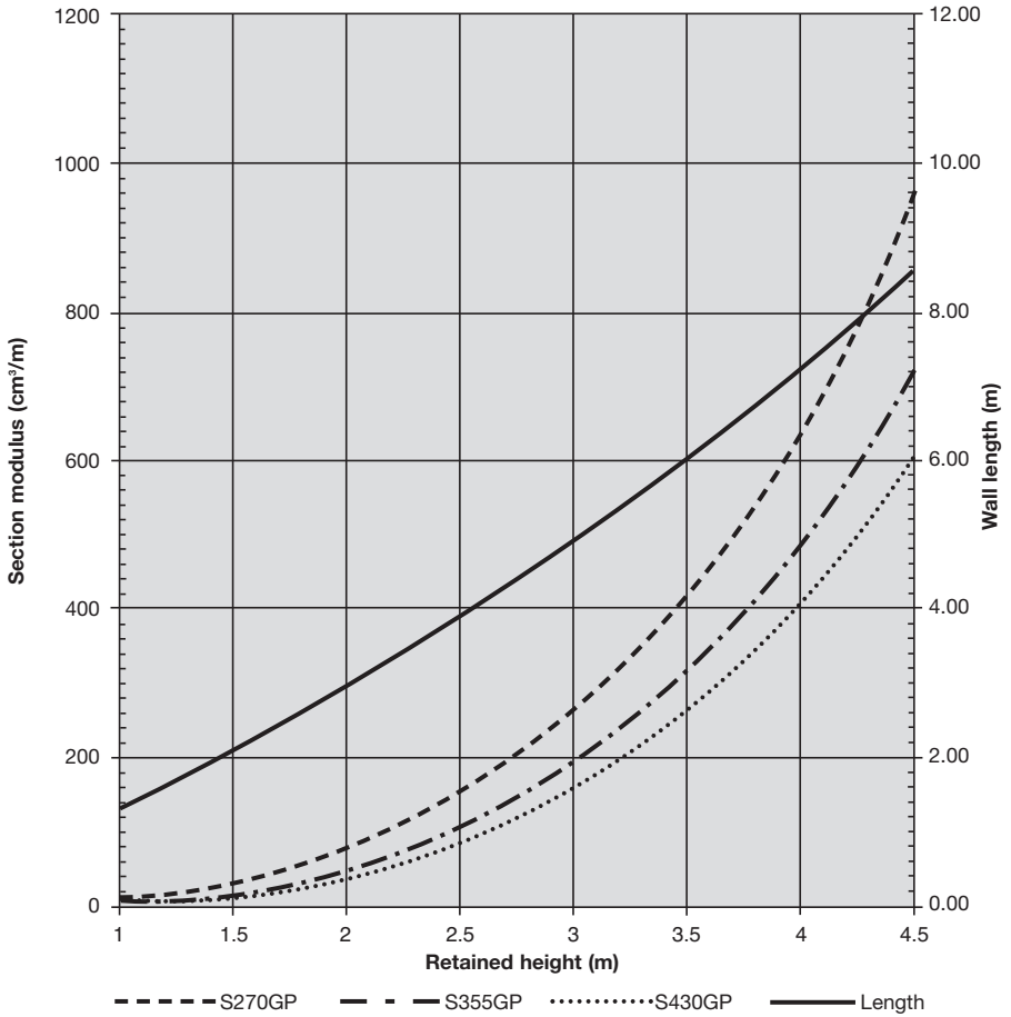
Fig. 8.30 Cantilever - Water condition D S_u = 75\text{kN/m}^2
