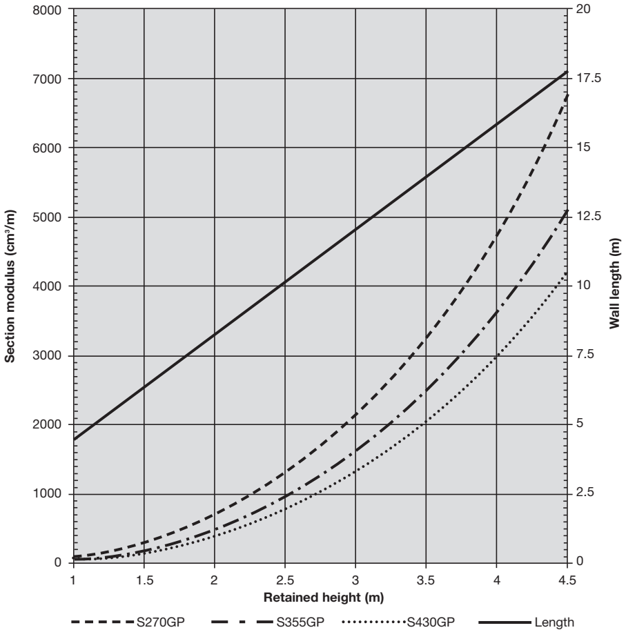
Fig. 8.11 Cantilever - Water condition A
