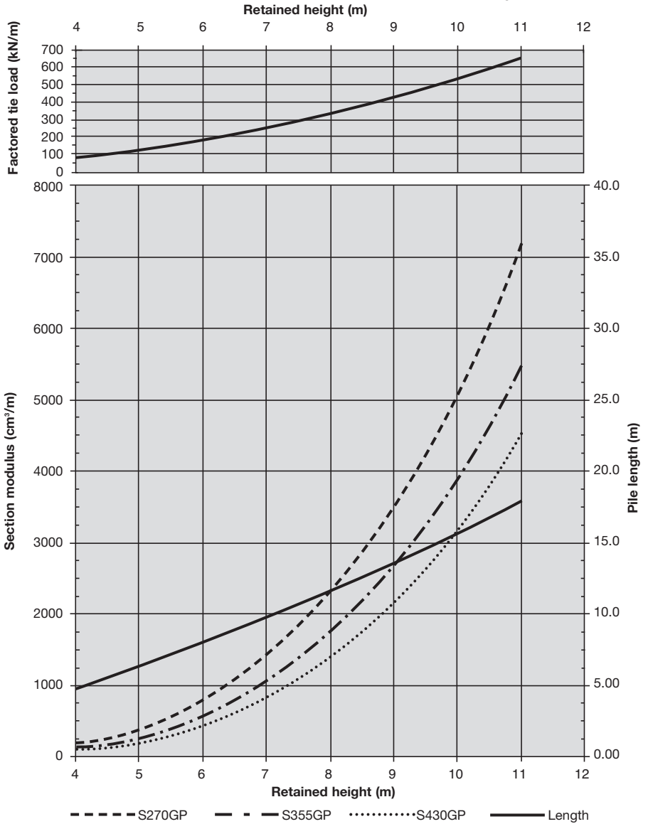
Fig. 8.34 Tied - Water condition D (d=1.2m) S u = 75kN/m 2
