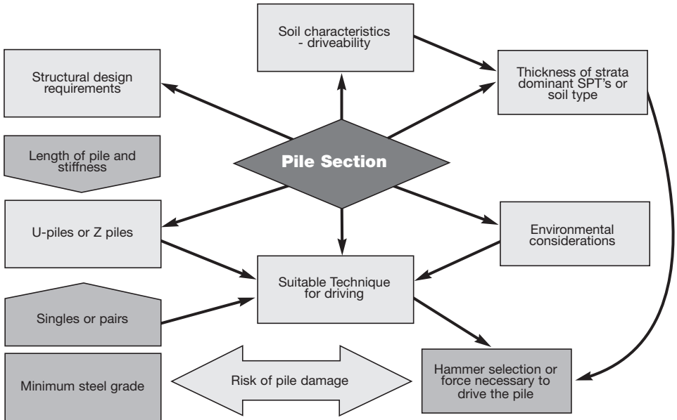
Figure 11.5.4 Summary diagram showing influences on choice of section
