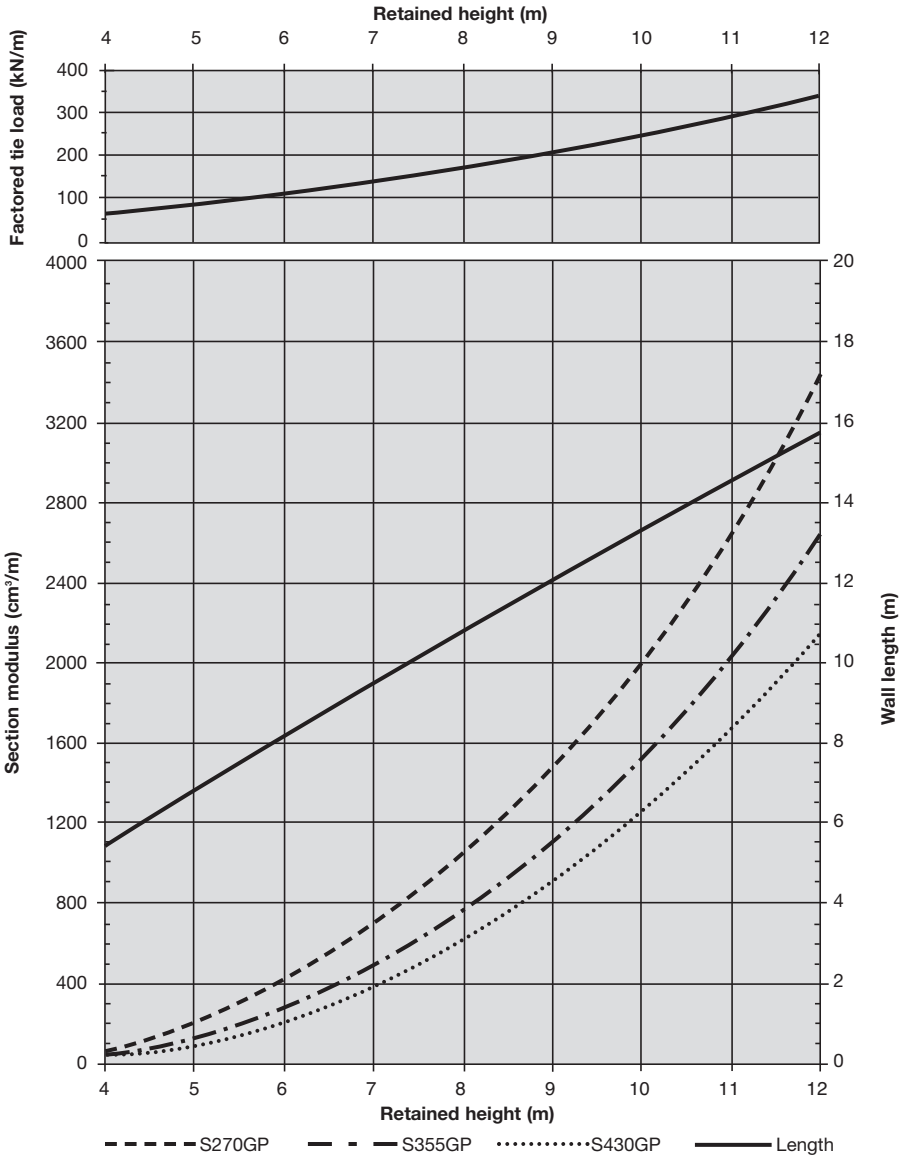
Fig. 8.22 Tied - Water condition B (d=1.5m)
