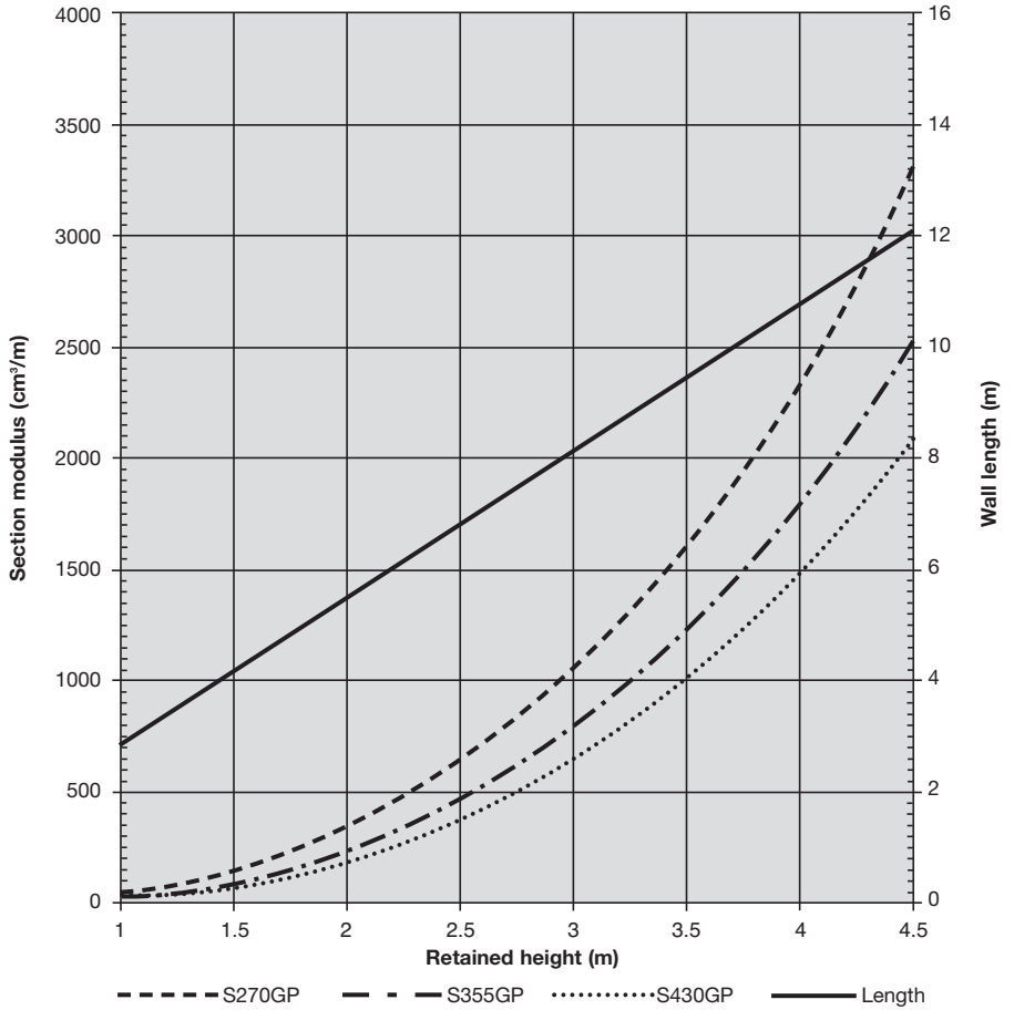
Fig. 8.10 Cantilever - Water condition A
