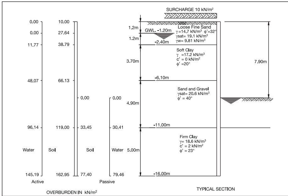
Fig 4.16.3 Effective Stress Analysis Example
