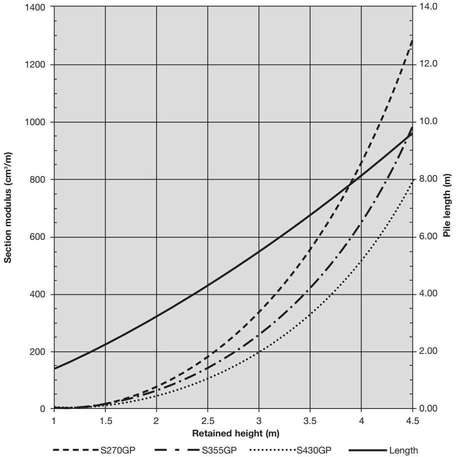
Fig. 8.28 Cantilever - Water condition C
