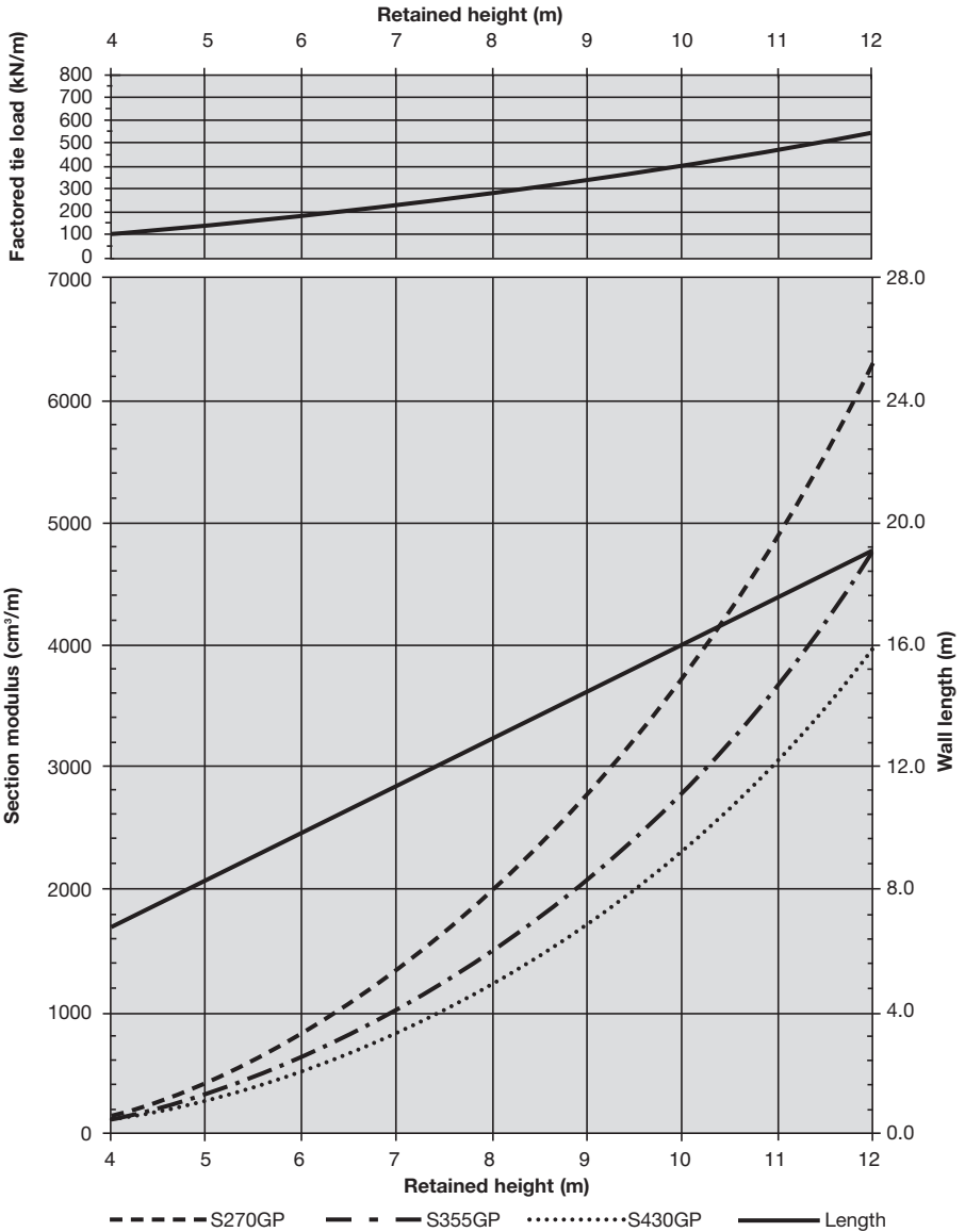
Fig. 8.23 Tied - Water condition B (d=1.5m)
