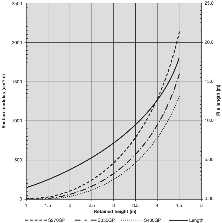
Fig. 8.29 Cantilever - Water condition C S_u = 40\text{kN/m}^2
