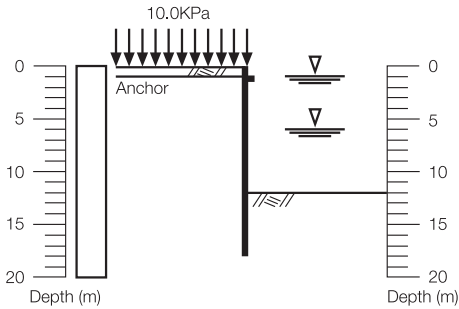
Fig 3.4a Design cross section
