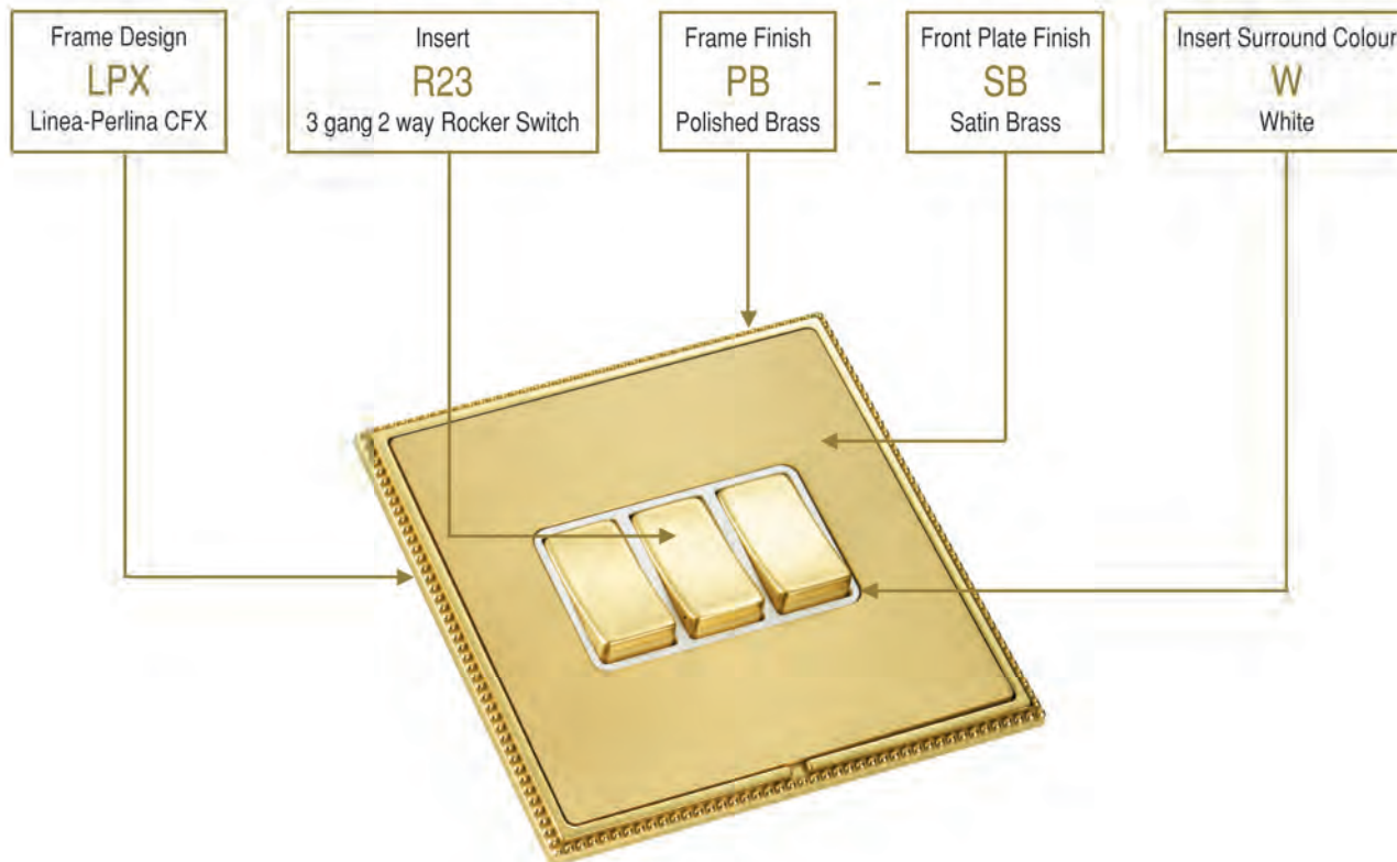
Illustration of Product Code configuration to order a Linea-Perlina CFX LPX R23 PB-SB W
