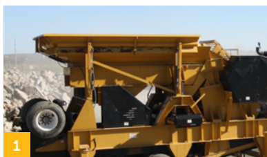
1 A 10.5 yd 3 hopper combined with the power of a C9.3B Caterpillar® Diesel Engine allows processing rates.
