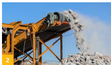
2 The 11' discharge height, one of the highest in the industry, allows not only superior stockpiling capabilities, but also the ability to pair it with screening units. An optional self-cleaning magnet extracts metals from processed material.
