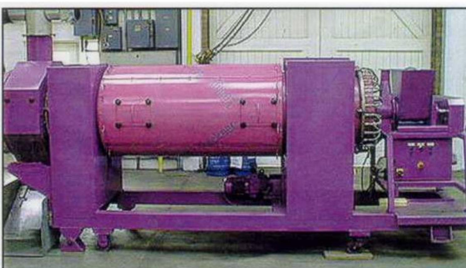
Pilot plant available for on-site client testing with approximately 80kgs/hour evaporative capability
