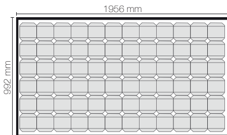
PLM-300P-72 Series/ PLM-300P-72 Series Weight: 21kg
