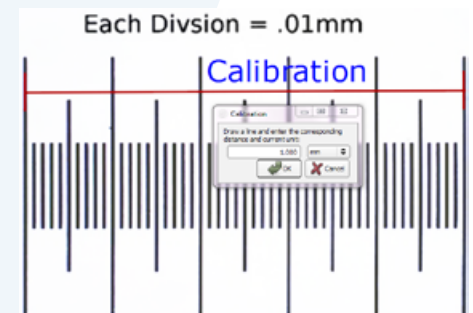
Calibration window
