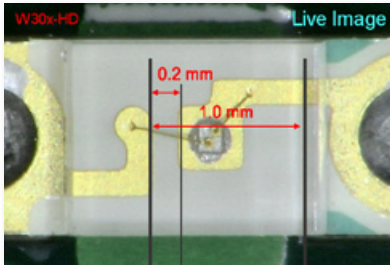
Overlay of Digital Graticule on live image
