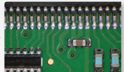
RingLight with 50% Crossed Polariser
