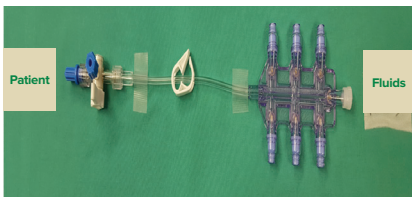
Figure 1: Set up of iv tubing, manifold, and downstream stopcock that could potentially allow for inadvertent aspiration if performed at the level of the stopcock and syringes are freely connected to the manifold.
