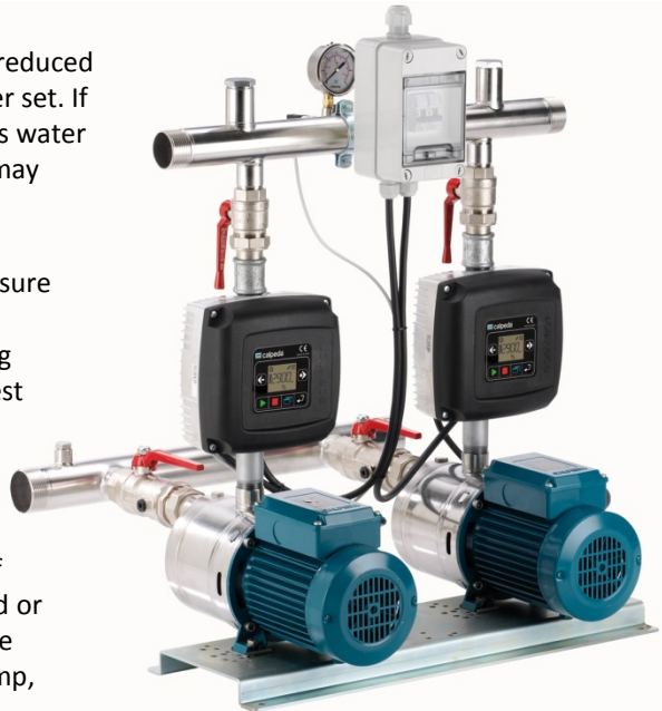
Twin pump booster set with horizontal multistage pumps and inverter drives
