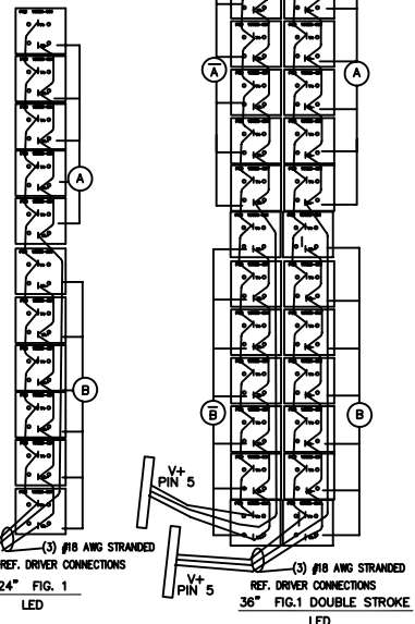
TYPICAL WIRE CONNECTION 24" FIG. 1 LED
