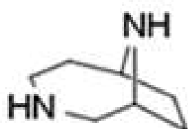
2 ring fused aliphatic
