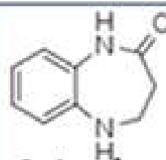
2 ring fused part saturated
