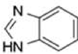
2 ring fused aromatic
