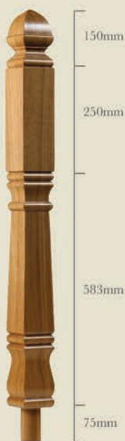
C9N0 2 Conkra Long Square Newel Post 983x91x91mm
