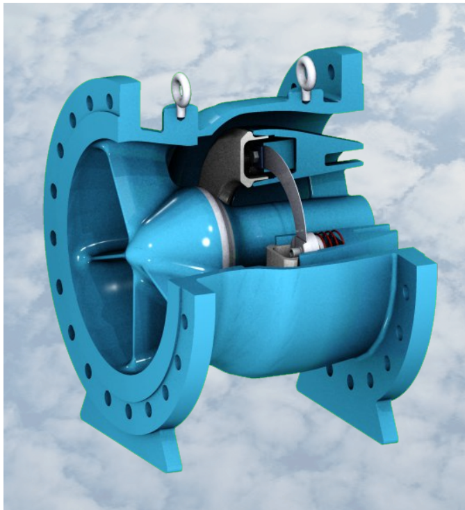
Vent-O-Mat ® NCV-B
