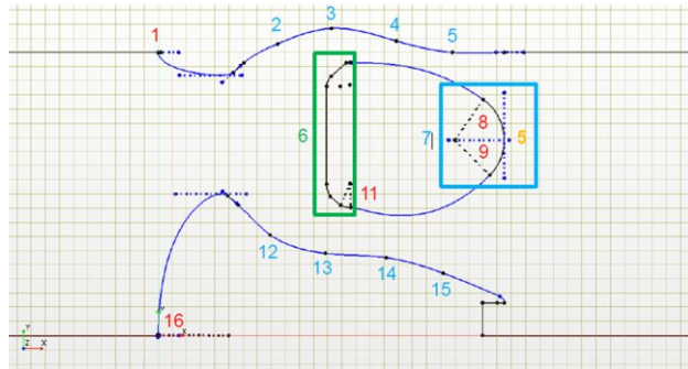
Parameterized 2D Axisymmetric Model
