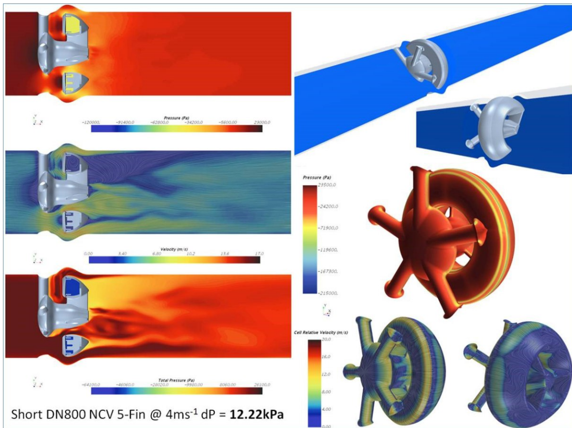
Images depicting the results of the CFD analysis and optimization
