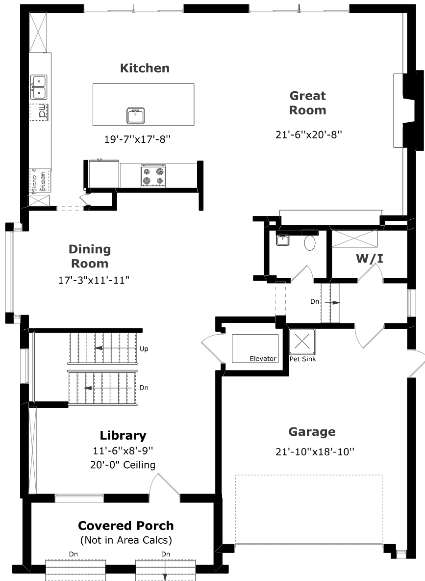
Main Floor Plan 1,716.8 sq. ft. + 414.8 sq. ft. (Garage) 9'-10" Ceilings
