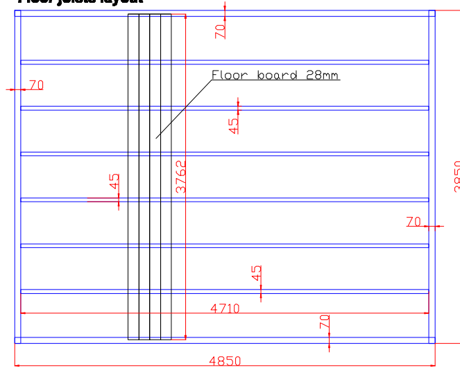
Floor joists layout
