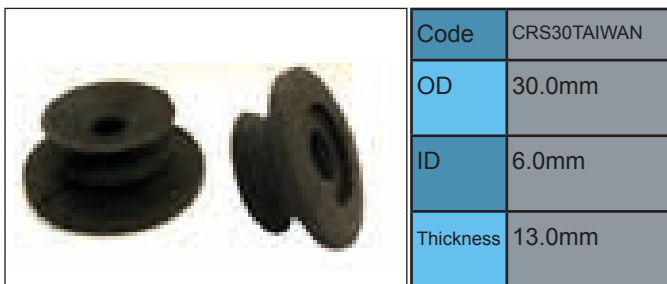
HEIDELBERG TAIWAN VERSION
