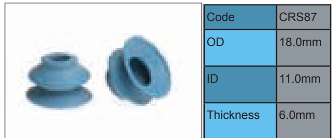
BONELLI FOLDER
