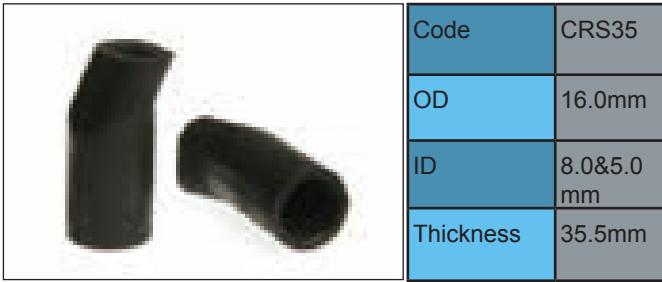
HAMADA #H05-49-01-3 CRS35S - SOFT VERSION
