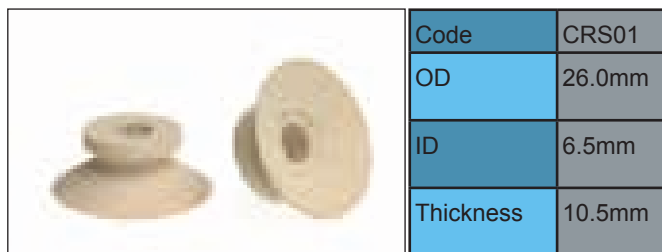
HARRIS 90LB / DIDDIE GLASER CRS01H - HEAVY DUTY CRS01T - THIN
