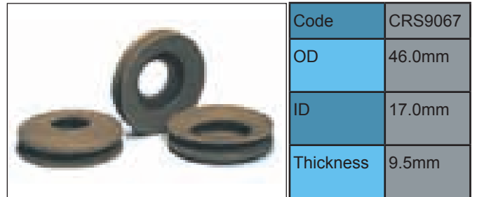
BOBST 9067
