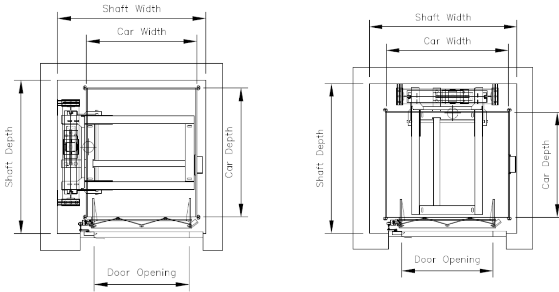
Cars with Bus Type Doors, Swing Hinge Landing Doors, Single Car Entrance, Ram to the side
