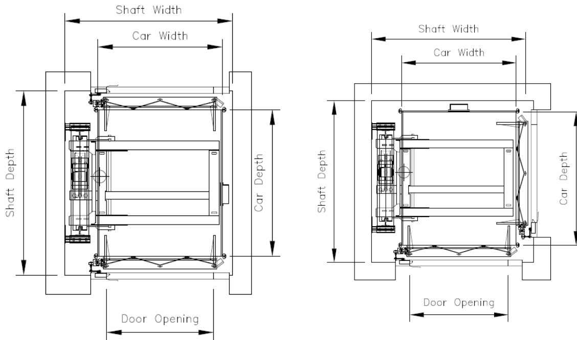
Cars with Bus Type Doors, Swing Hinge Landing Doors, Through Car, Ram to the side
