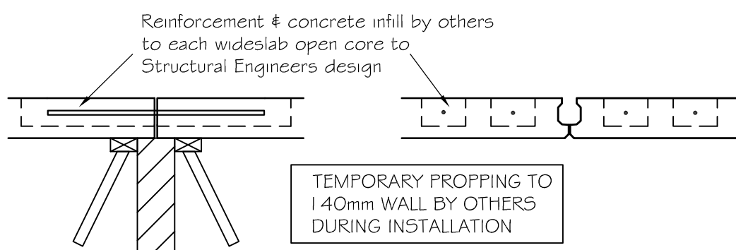
140mm SHARED BEARING WALL DETAIL
