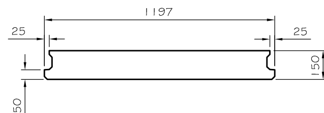
150mm DEEP WIDESLAB DIMENSIONS
