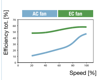
Fig. 2: Efficiency
