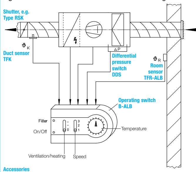
Fig. 1: Functional overview ALB EH with electric heating
