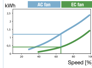
Fig. 3: Energy consumption in controlled operations
