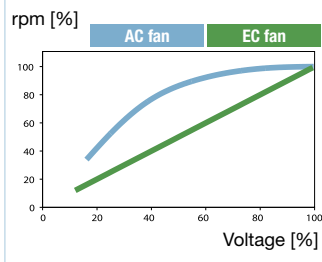
Fig. 1: Speed regulation
