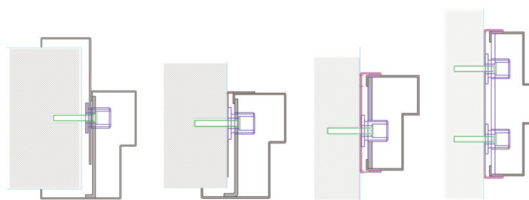
Type A Type B Type C Type D Types A & B available in both Inward & Outward Opening Versions.
