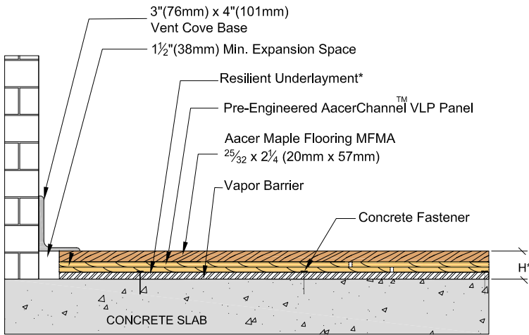
Wall Base
