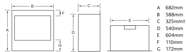
Atina HE with log fuel effect and Wide trim in antique brass.
