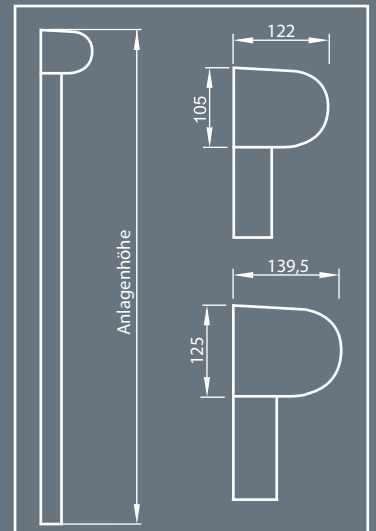
The round system SolidScreen® SGF
