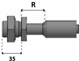
Bulkhead male insert O-ring, straight
