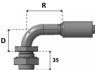
Bulkhead male insert O-ring, , 90° elbow
