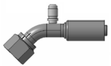
O-ring female swivel - pressure sensor 7/16-20 45° elbow
