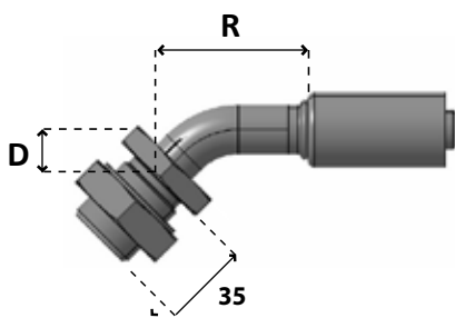
Bulkhead male insert O-ring, , 45° elbow
