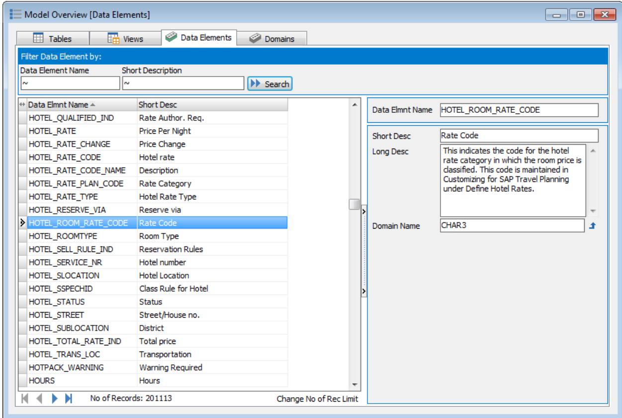
Model Overview: Data Elements
