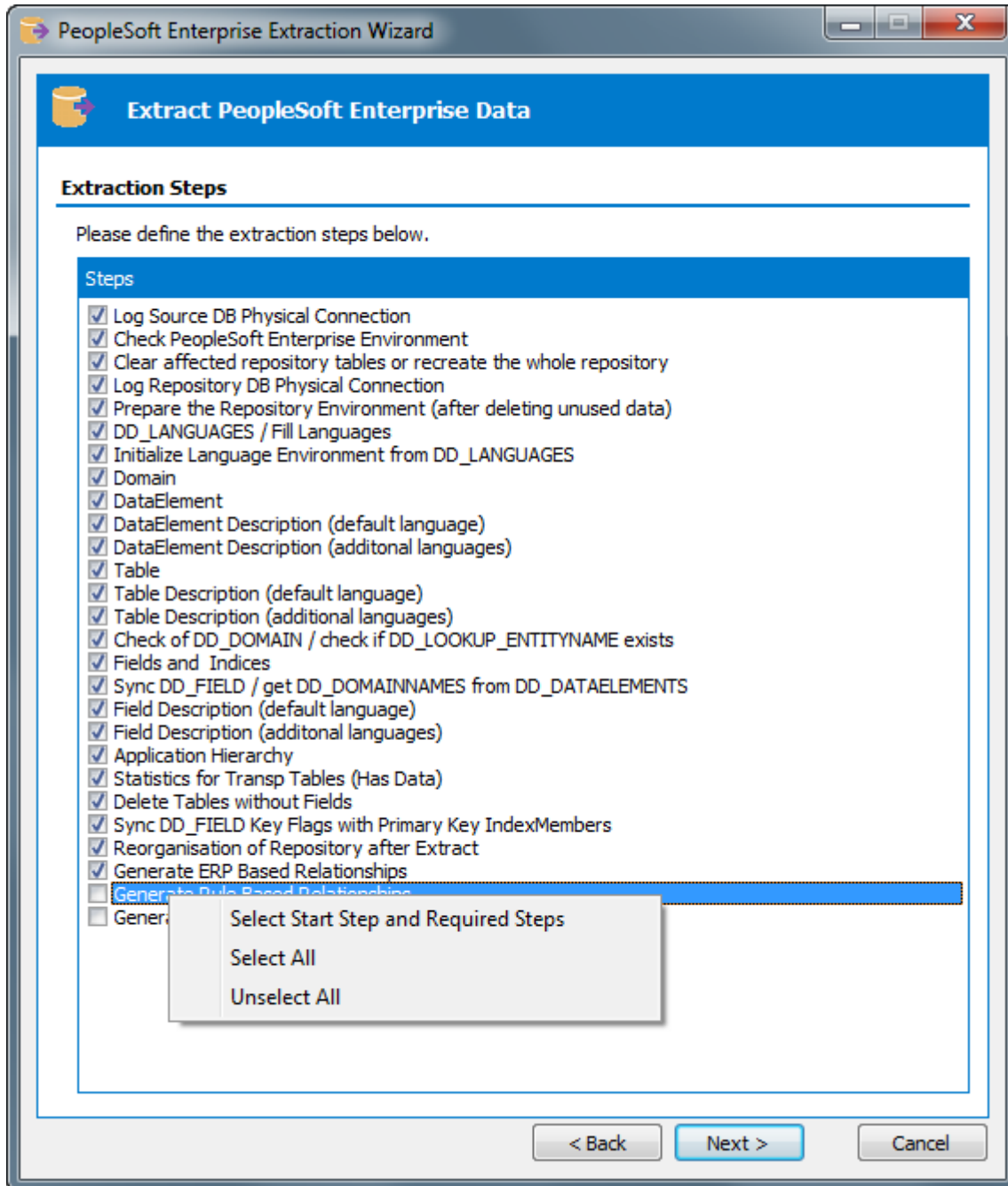
Using Right Mouse click to select the Starting Step for Extraction
