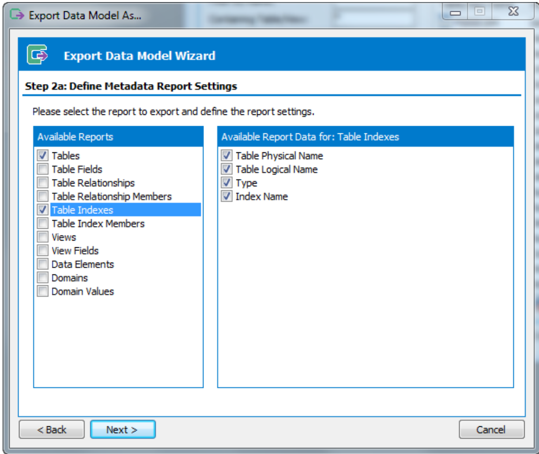
Metadata Report Settings
