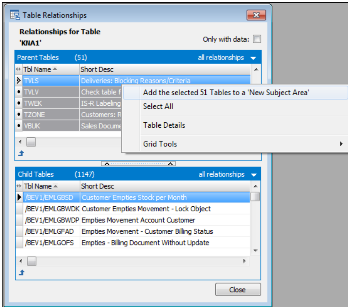
Adding related tables to a new Subject Area
