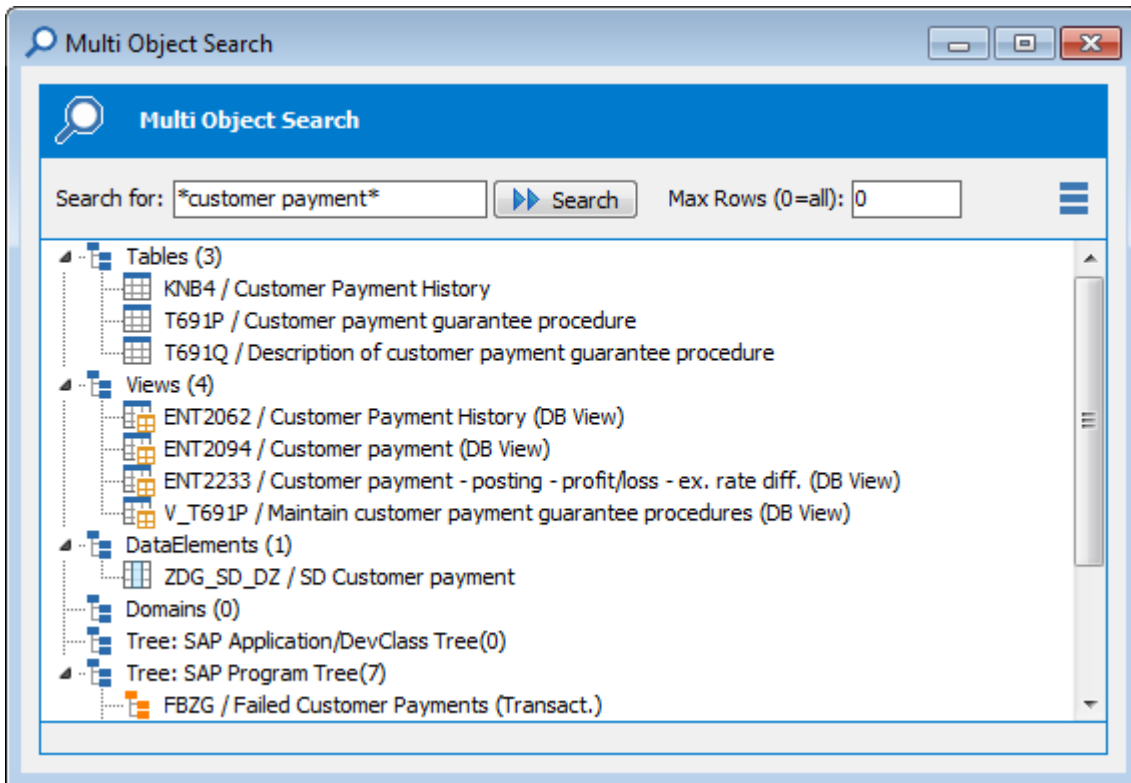
Multi-Object Search showing result details
