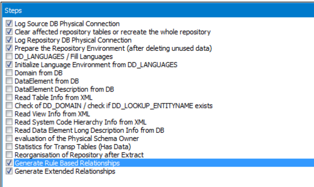
Setting the extraction options to only run the 'Generate Relationships' process
