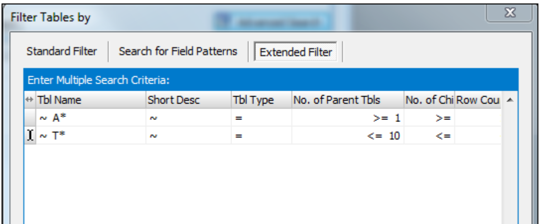
Example with multiple selection lines
