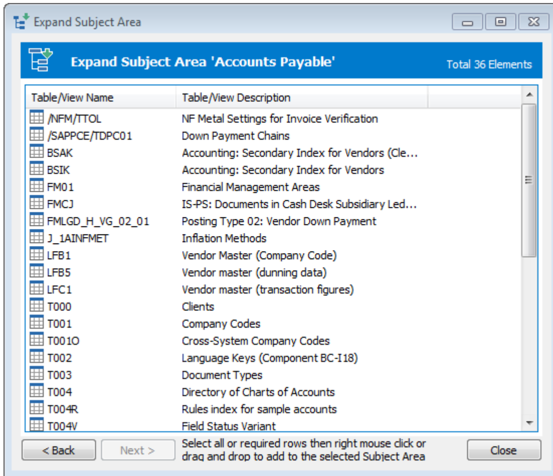
Result set from using the Expand Subject Area feature
