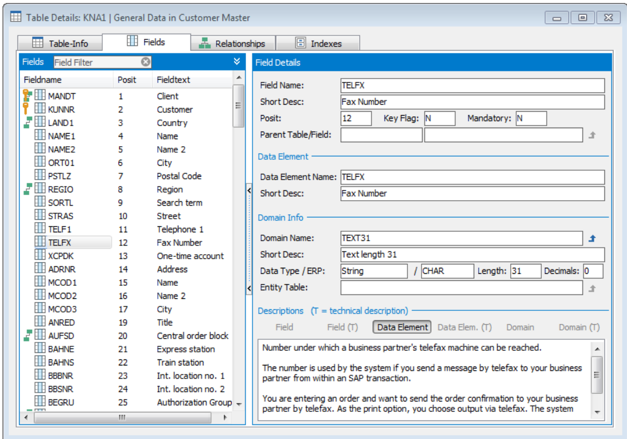
Displaying Field Details
