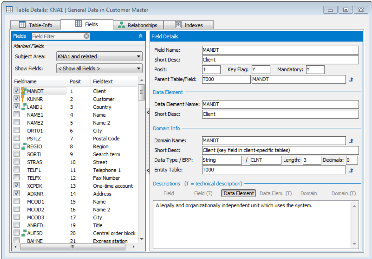
Marked Fields options on Table Display
