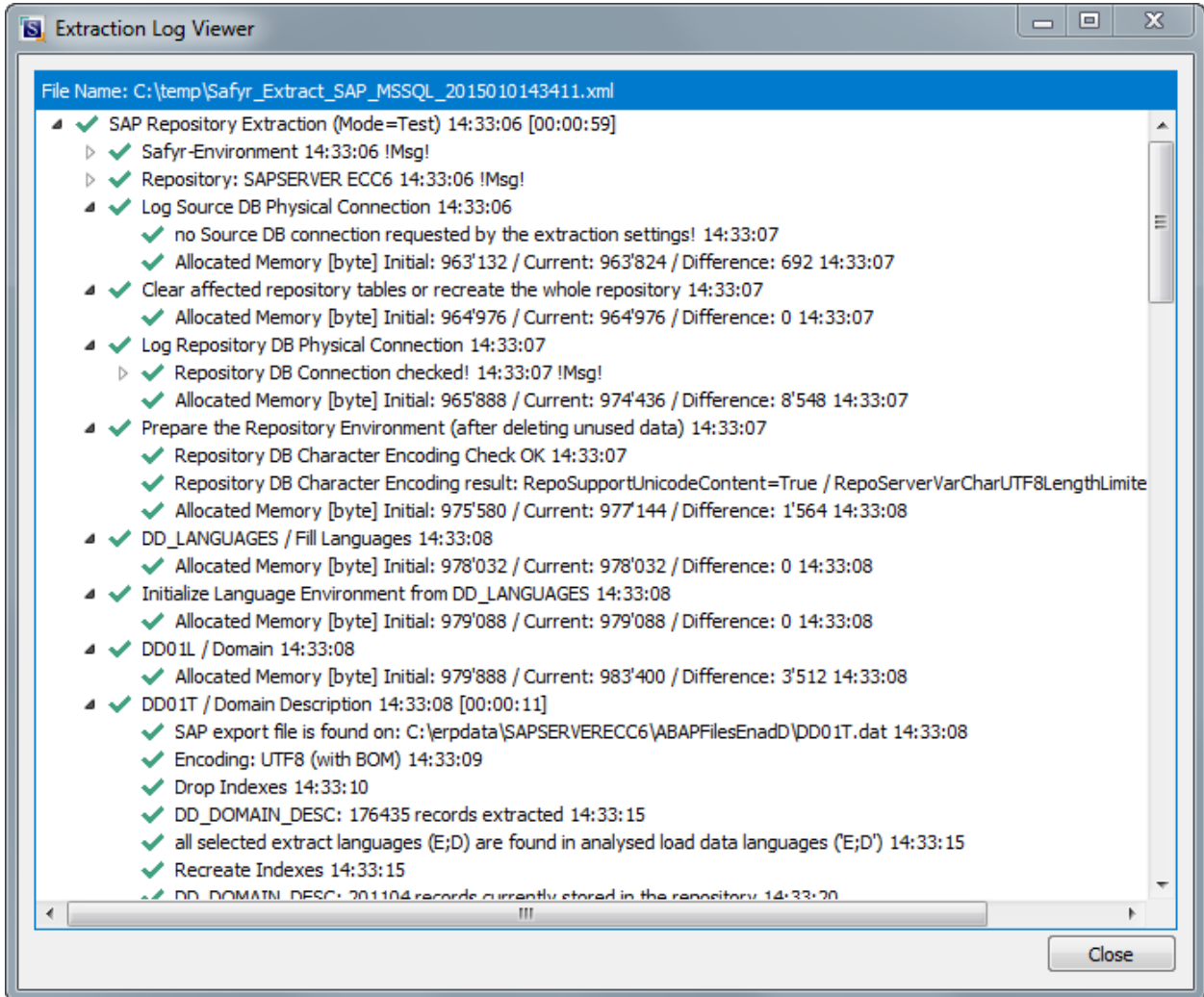
Viewing the Extract Log
