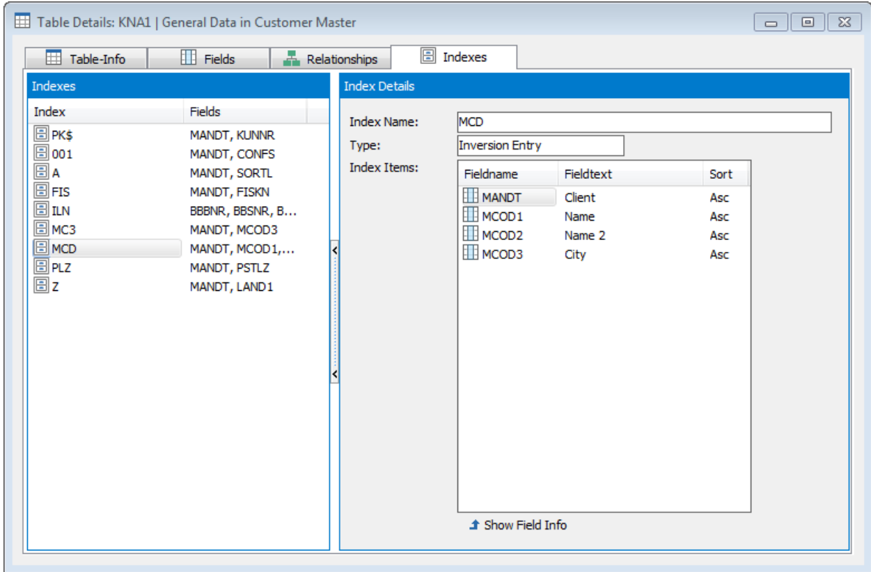
Viewing Index Information
