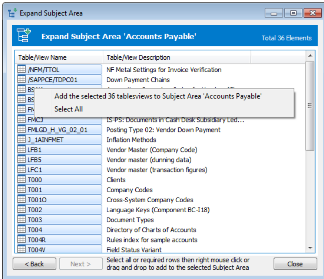
Using the Right Mouse Click menu to select and then add the relationships to a Subject Area
