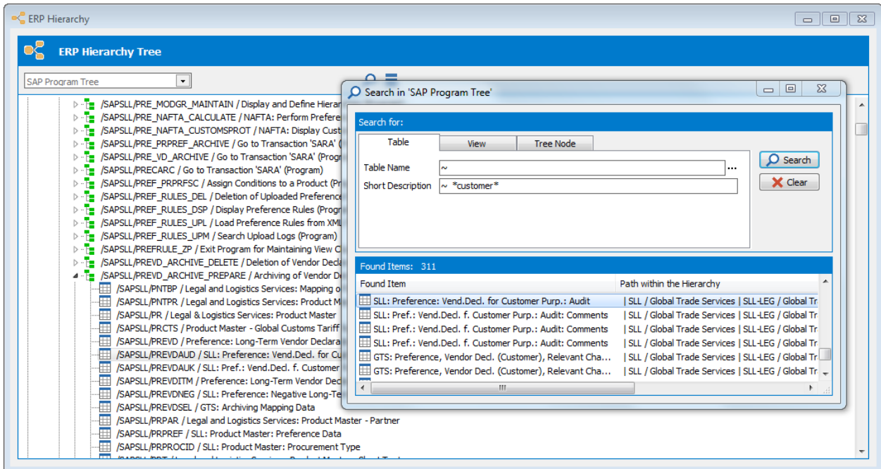
Using the Search Tables result to locate a table in the Hierarchy
