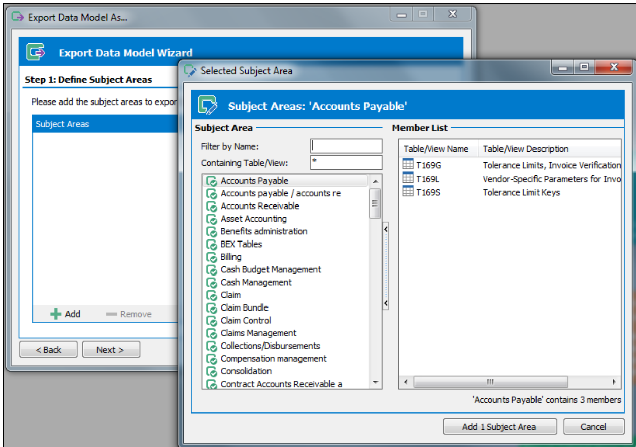
Adding Subject Areas to be exported
