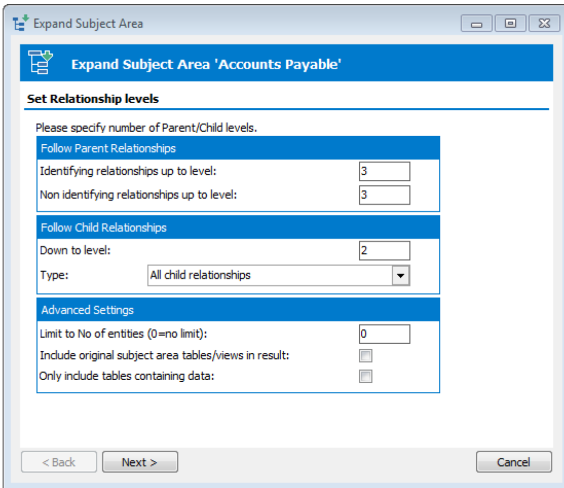
Specifying levels of tables to be included in a Subject Area expansion
