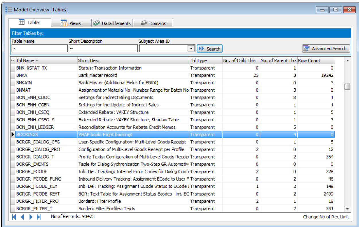
The Model Overview form
