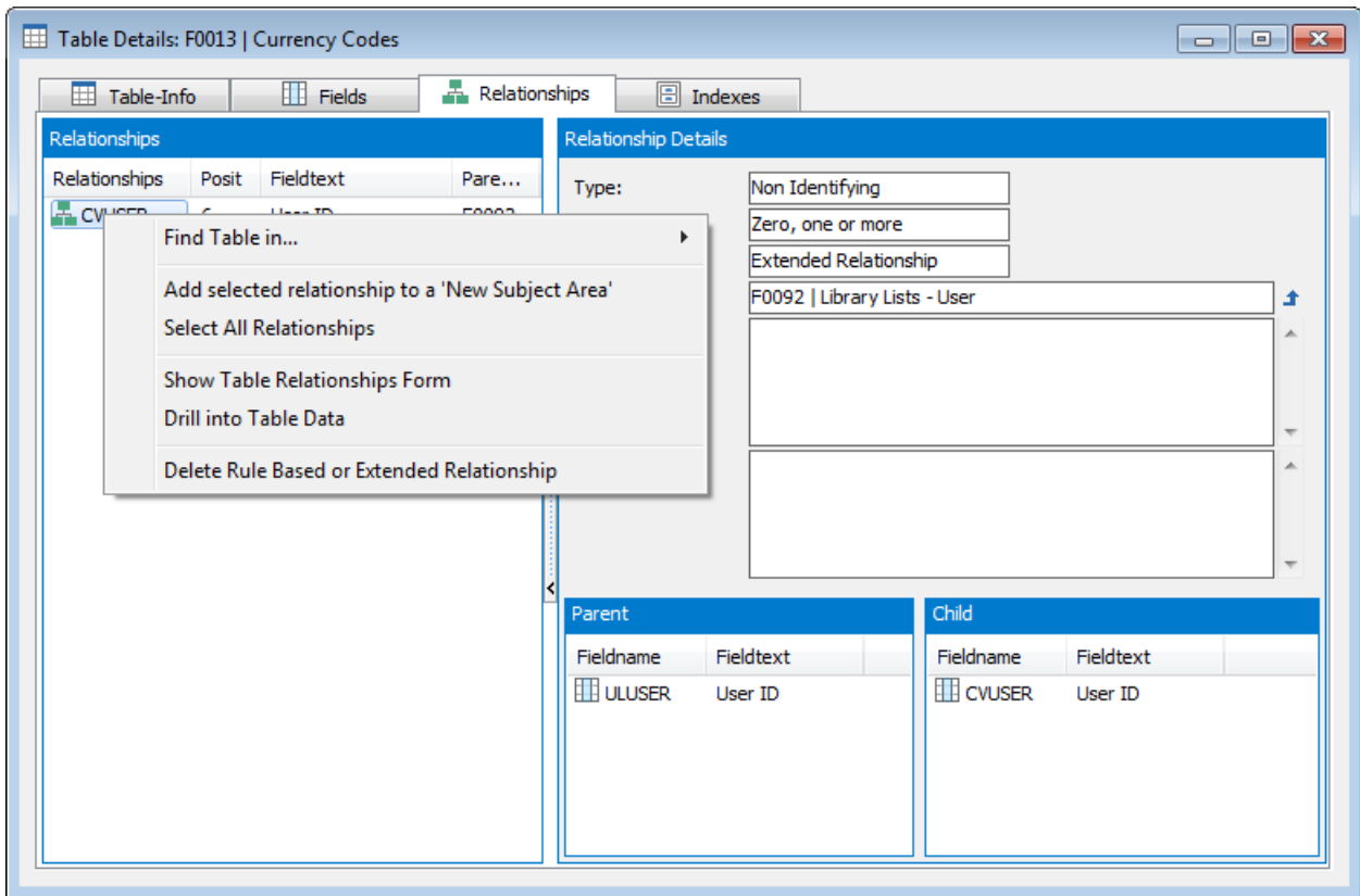
The Rules based/Extended Relationship Delete Pop-up
