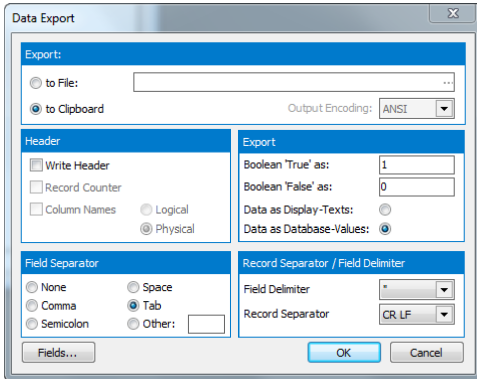
Export table List screen
