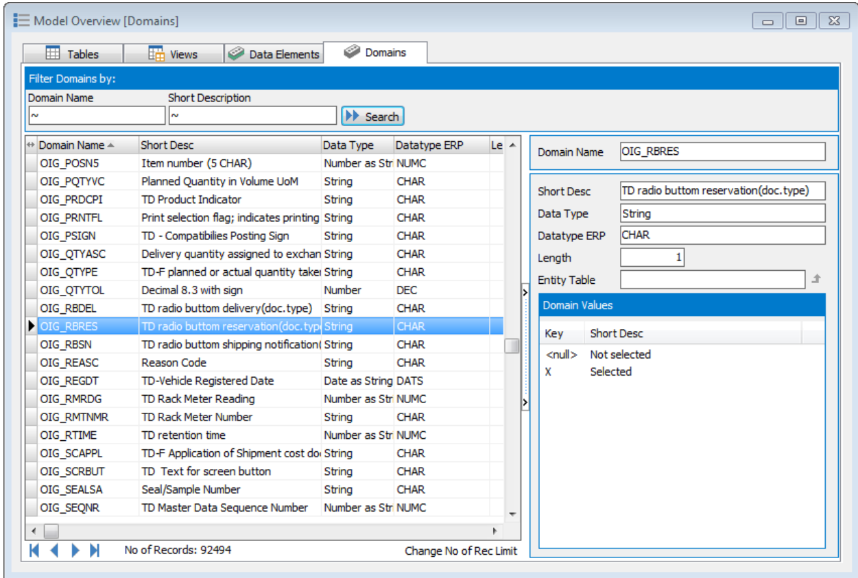
Model Overview: Domains
