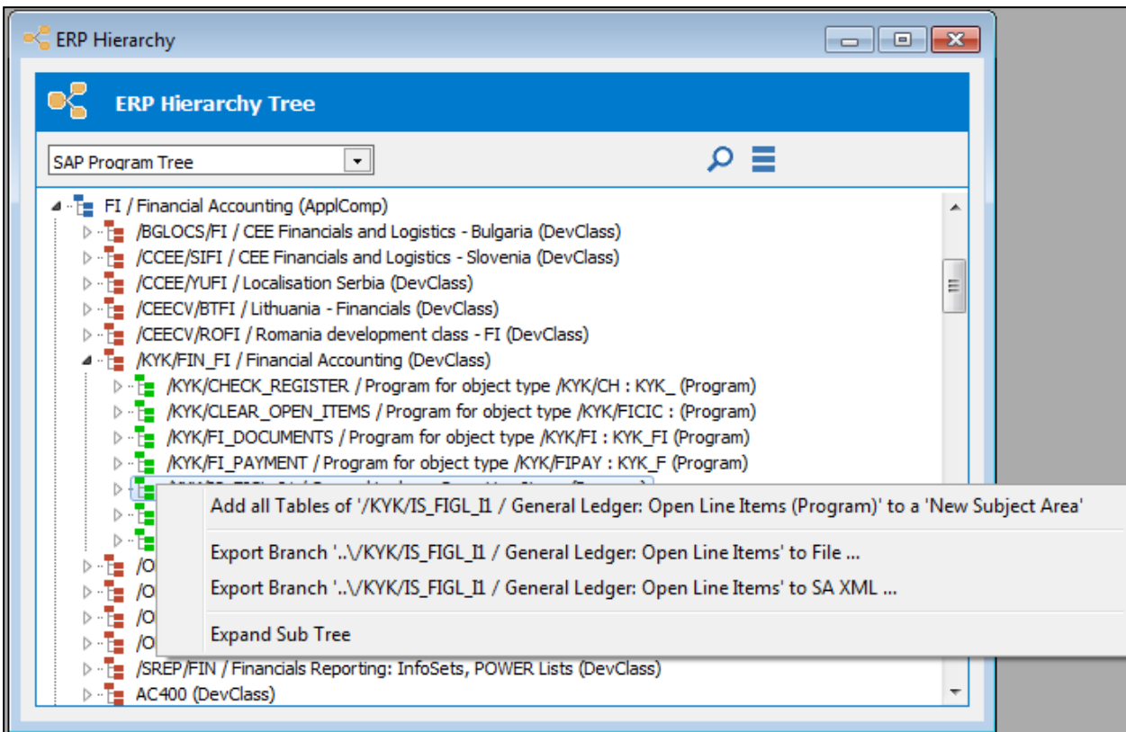
Populating a new Subject Area from the Application Hierarchy
