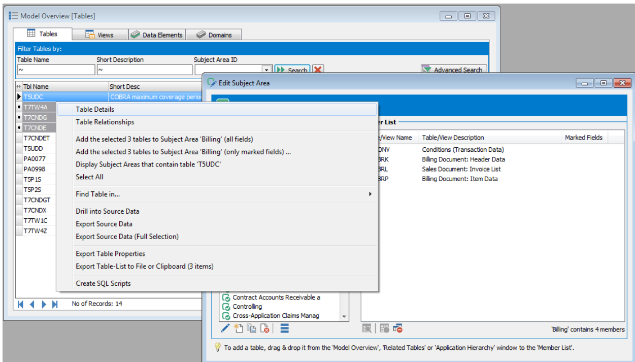
Populating an existing Subject Area from the Model Overview
