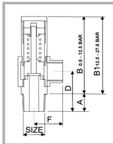
Dimensions in mms
