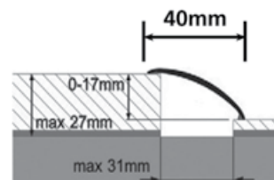
WRG2 REDUCER SELF ADHESIVE 900mm & 1800mm All Colours
