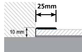
WRG3 EDGE SELF ADHESIVE 1800mm All Colours
