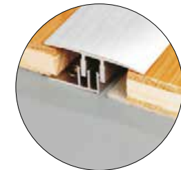
Transition 588 2-Part Screw Down Silver 2700mm 10mm - 16mm F1627005
