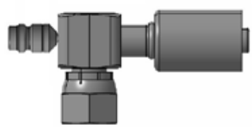
Short drop O-ring swivel - 90° block type - R134a valve - forward
