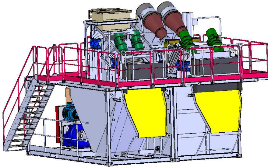
Dredge complete desanding plant (size and configuration are not contractual)
