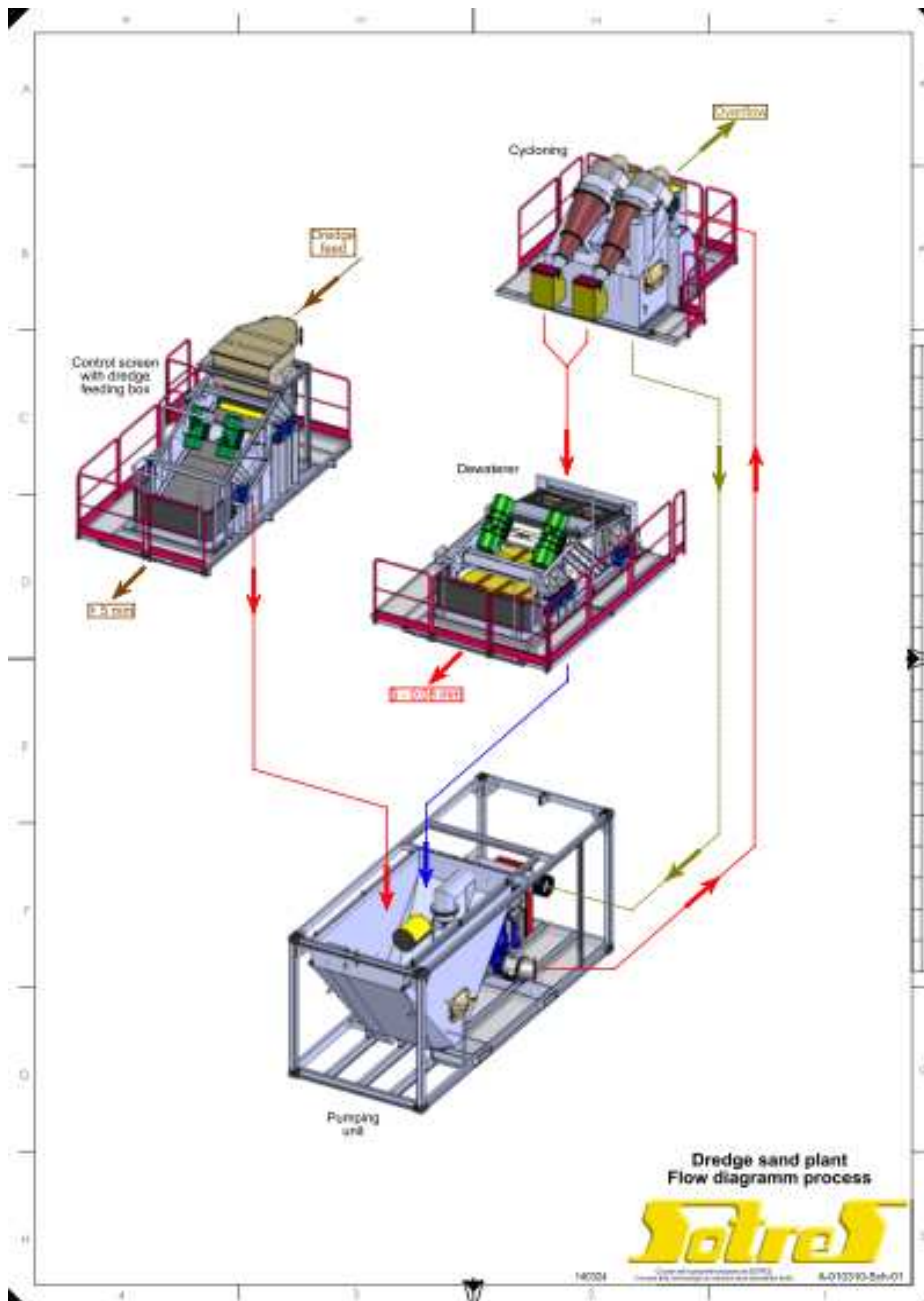
Dredge desanding plant Flowsheet
